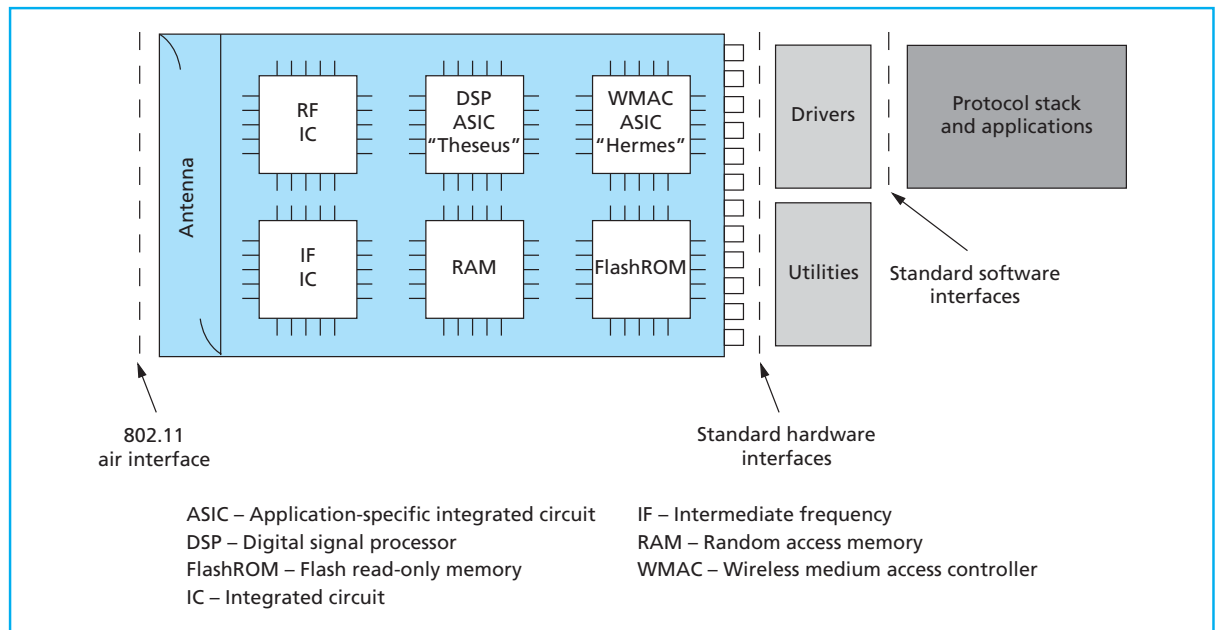
Figure 2. Major WaveLAN-II functions.
