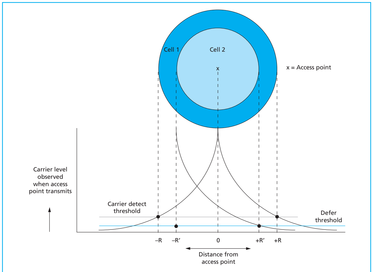
Figure 10. Large cell characteristics.
