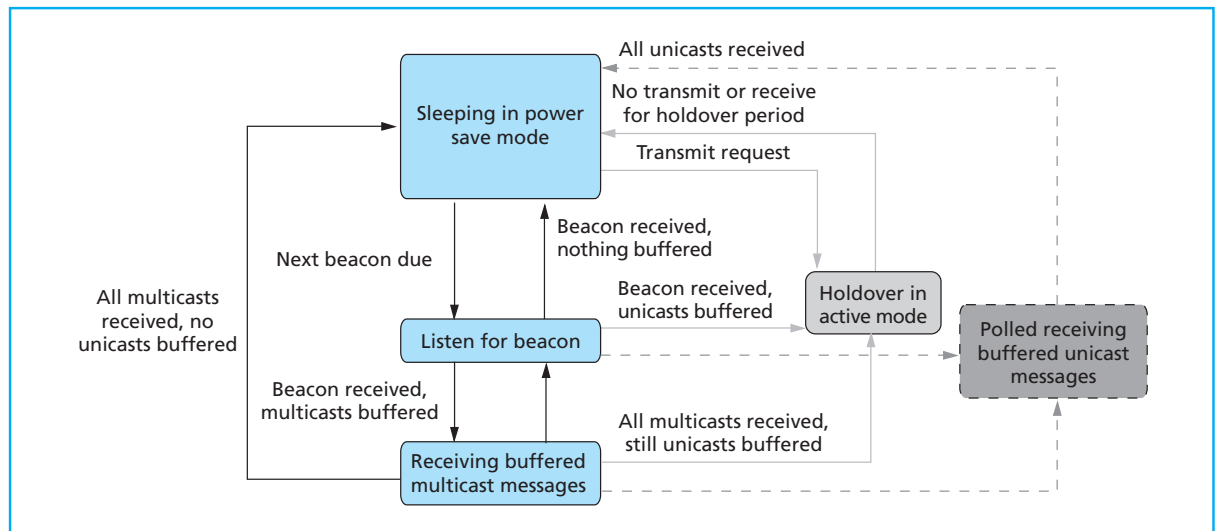
Figure 7. State diagram for two different power management schemes.
