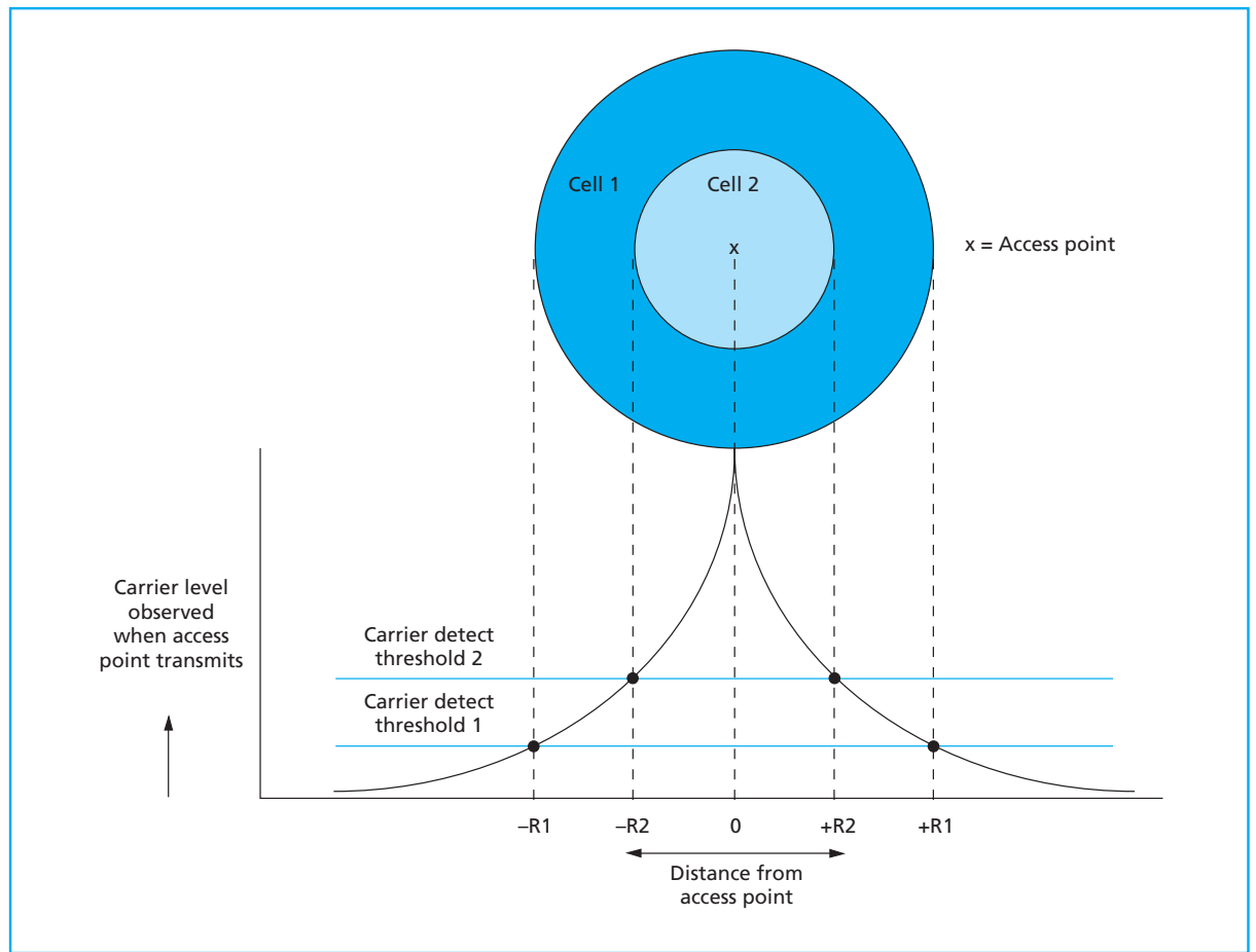
Figure 8. The effect of carrier detect threshold on cell size.
