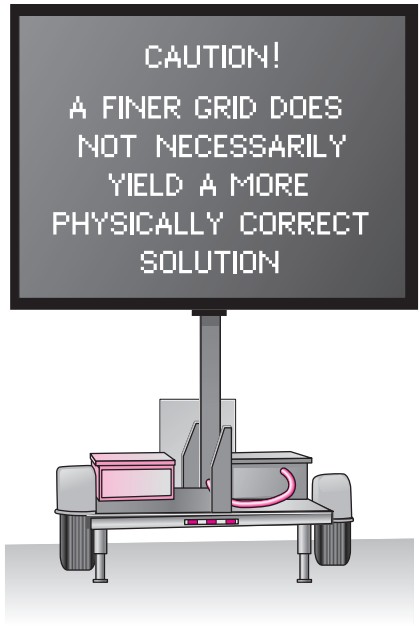
FIGURE 15–41 Poor grid resolution can lead to incorrect CFD results, but a finer grid does not guarantee a more physically correct solution. If the boundary conditions are not specified properly, the results may be unphysical, regardless of how fine the grid.
