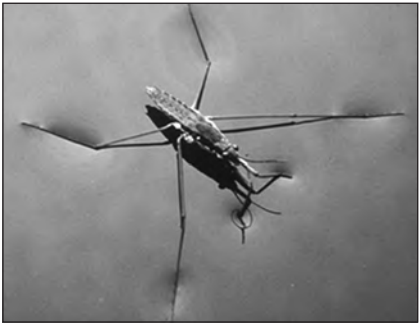
FIGURE 7-2 The water strider is an insect that can walk on water due to surface tension. © Dennis Drenner/Visuals Unlimited.
