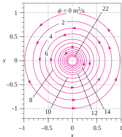
FIGURE 9-27 Streamlines for the velocity field of Example 9-12, with K = 10 \text{ m}^2/\text{s} and C = 0 ; the value of constant \psi is indicated for several streamlines.
