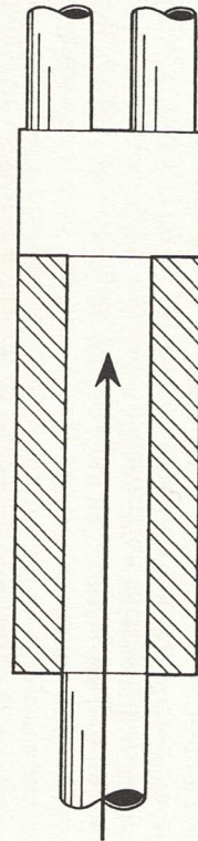
Fig. 6:8. Chamber incorporated in main body may improve silencing at periods of resonance, and also facilitate use of twin tailpipes.
