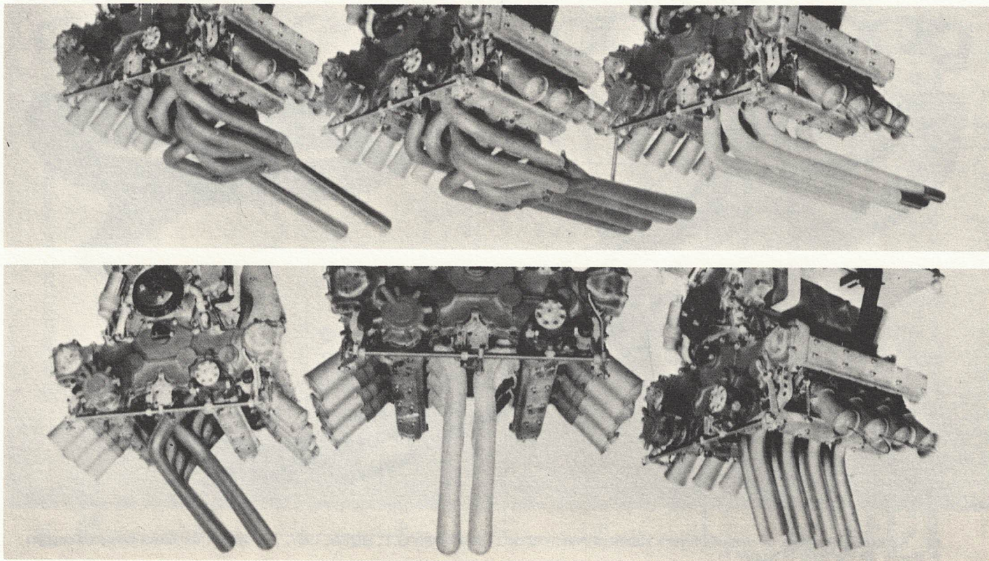
12 Various experimental exhaust systems employed when developing the Ford V-8 racing engine with two-plane crankshaft (Chapter 8)
