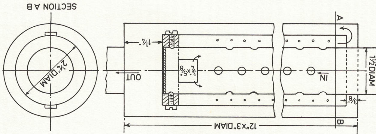
Fig. 6 : 15. The three-inch interference silencer.
