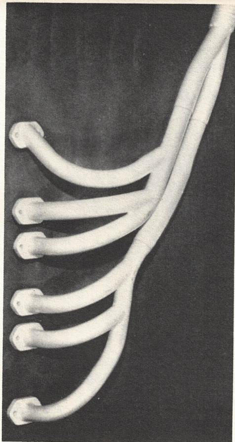
9 Manifold design for 'interference' working on six-cylinder engine (Chapter 7)
