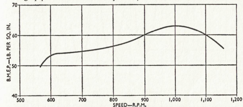
Fig. 5:15. Torque-speed curve of self-induction engine.
