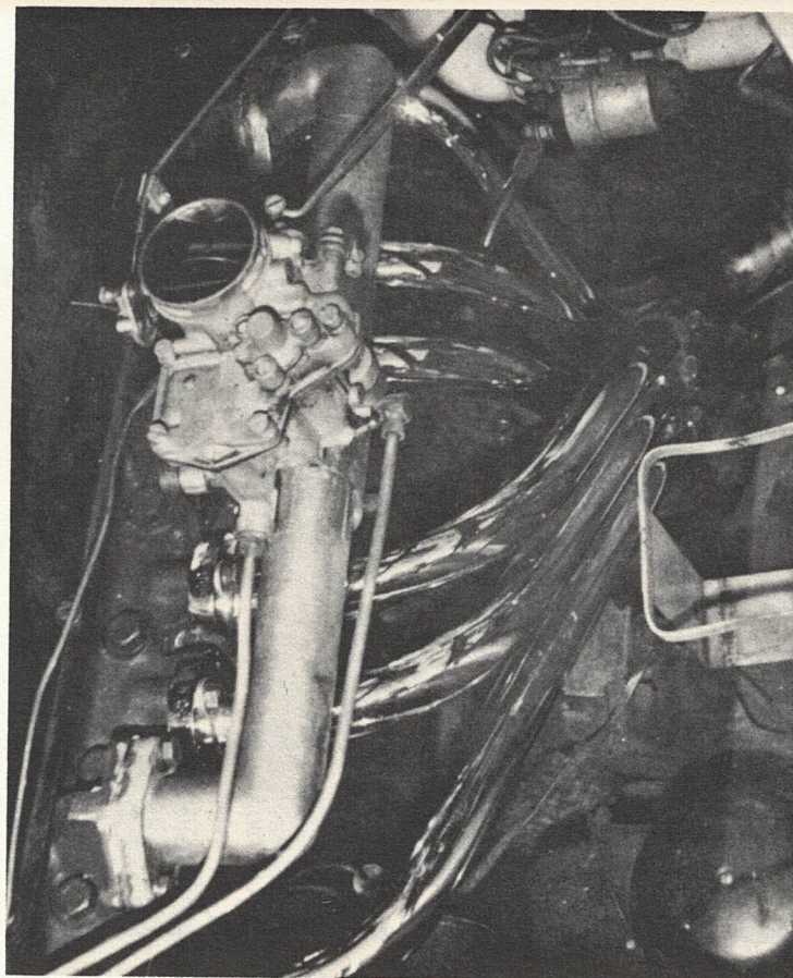
10 Manifold design for 'independence' working on six-cylinder engine (Chapter 7)
