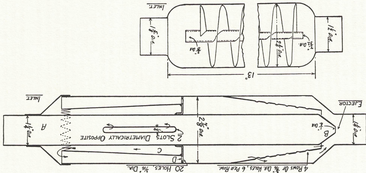
Fig. 6 : 10. Two types of back-pressure silencer of good design. Top - Scott-Howarth; bottom - Carbjetor.
