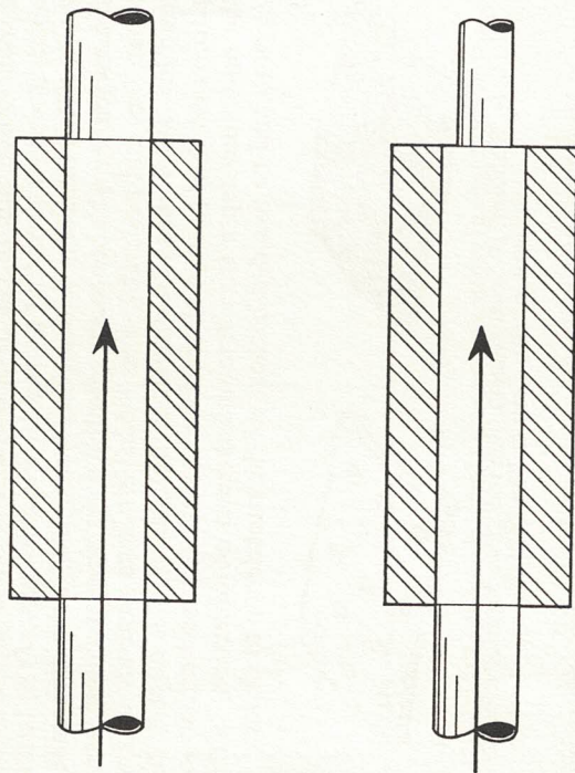
Fig. 6:7. Constant diameter throughway (top) gives minimum flow resistance, but reduced diameter outlet (bottom) adds to silencing effect.
