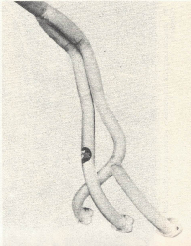
7 Manifold design for 'interference' working on four-cylinder engine with stamessed centre port. There is adequate pipe length before final junction (Chapters 5 and 7)
