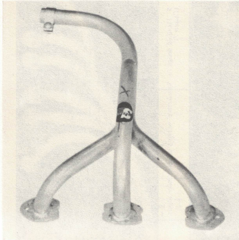
8 Manifold design for 'interference' working on four-cylinder engine with stamessed centre port (Chapters 5 and 7)
