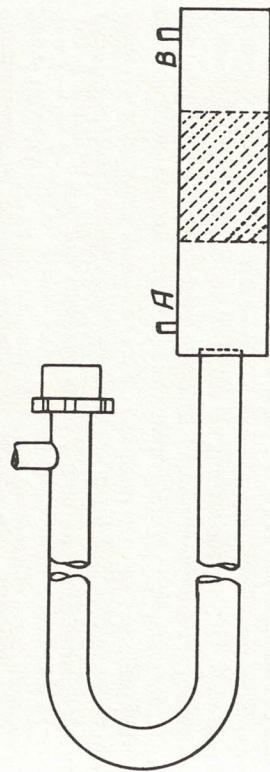
Fig. 6 : 17. Rig for testing pulse penetration.
