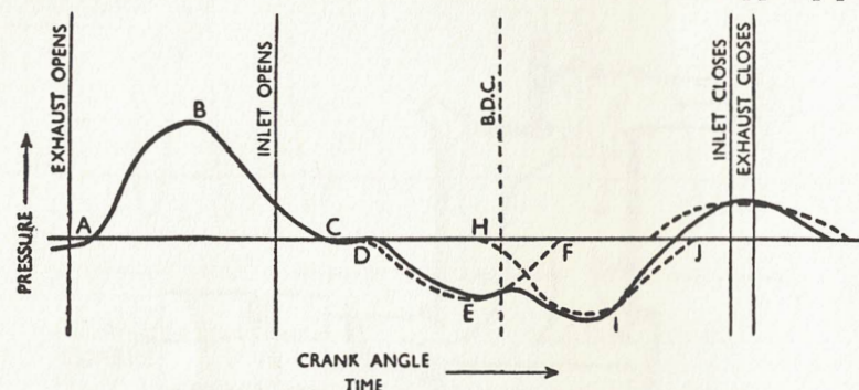
Fig. 5:14. Pressures in stepped exhaust pipe of self-induction engine.
