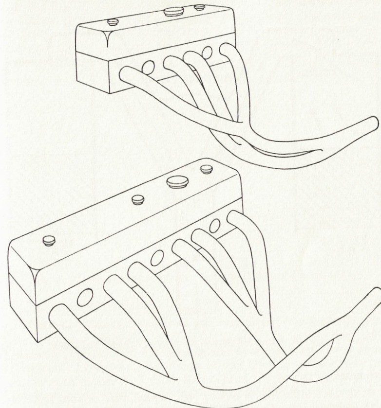
Fig. 5:18. Sub-division in manifolds to obtain equal discharge intervals at junction of branches.
