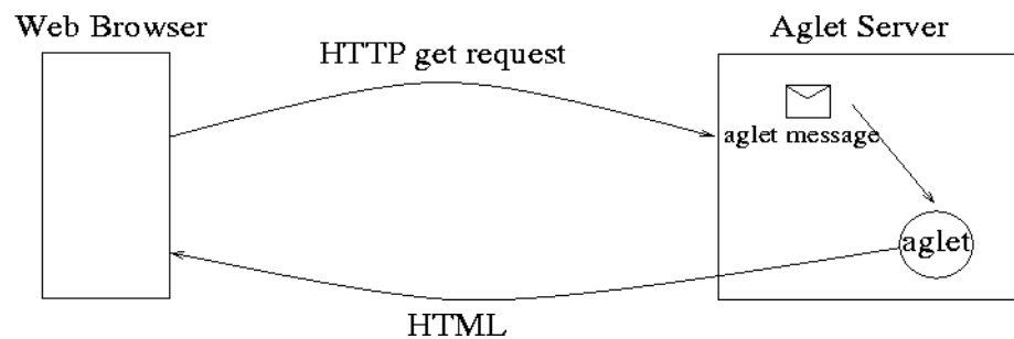
Fig. 6. Message-flow in HTTP Messaging
