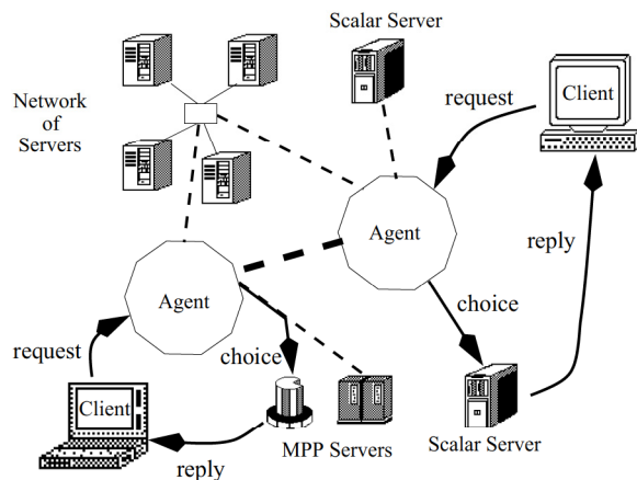
Figure 2: Basic structure of NetSolve
