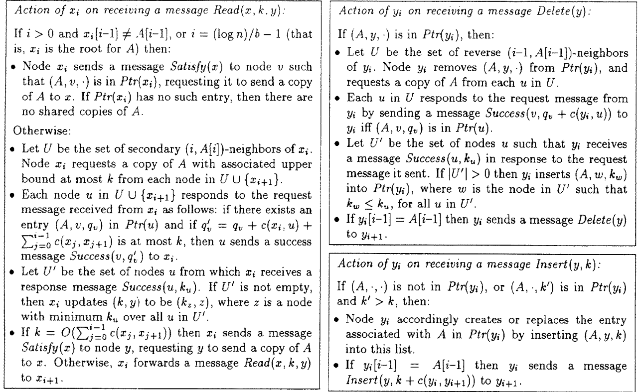
Figure 1: Actions on receiving messages Read , Insert , and Delete for object A .
