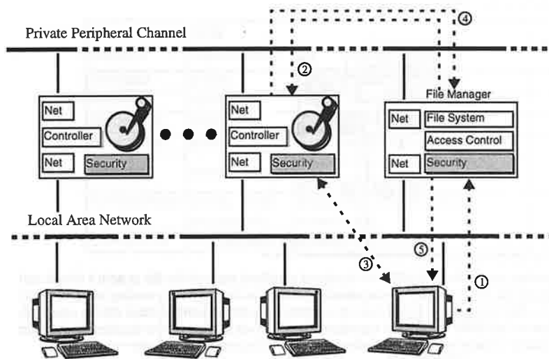
Figure 2: Network SCSI (NetSCSI) is a network-attached disk architecture designed for minimal changes to the disk's command interface. However, because the network port on these disks may be connected to a hostile, broader network, preserving the integrity of on-disk file system structure requires a second port to a private (file manager-owned) network or cryptographic support for a virtual private channel to the file manager. If a client wants data from a NetSCSI disk, it sends a message (1) to the distributed file system's file manager which processes the request in the usual way, sending a message over the private network to the NetSCSI disk (2). The disk accesses data, transfers it directly to the client (3), and sends its completion status to the file manager over the private network (4). Finally, the file manager completes the request with a status message to the client (5).
