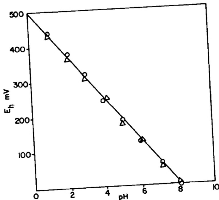
Fig. 4. Plot of E_h against pH (○—○, using quinhydrone electrode and \Delta — \Delta , using charcoal sample degassed at 500^\circ\text{C} and treated with hydrogen at 160^\circ\text{C} ).
