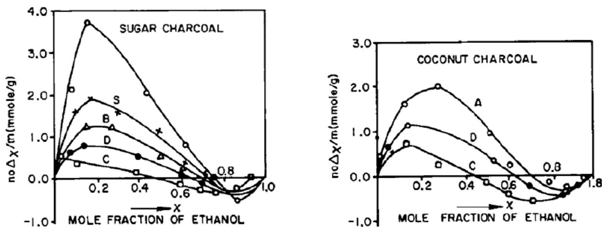
Fig. 10. Composite adsorption isotherms for various samples of charcoal from sugar and coconut shell and silica gel from ethanol-benzene mixtures. Curves A, original charcoals; B, outgassed at 400°C; C, outgassed at 750°C; D, outgassed at 1100°C; S, silica gel.
