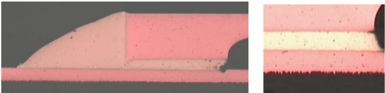
Figure 10: Cross-section views of a mounted VDSO package. The left photo shows a SAC305 solder joint of a small pad (gate/source). The right photo shows the outer edge of a drain pad which in case of VDSO is comparable to the inner edge.
