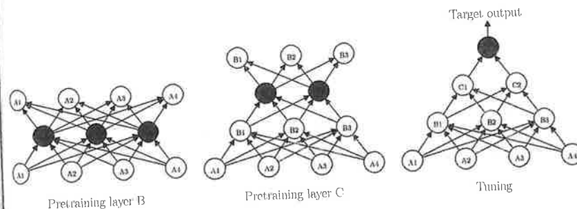
Figure 4.5 The pretraining and tuning stages in greedy layer-wise pretraining. Black circles represent the neurons whose training is the primary objective at each training stage. The gray background marks the components in the network that are frozen during each training stage.
