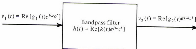
FIGURE 4-2 Filtering bandpass waveforms.
