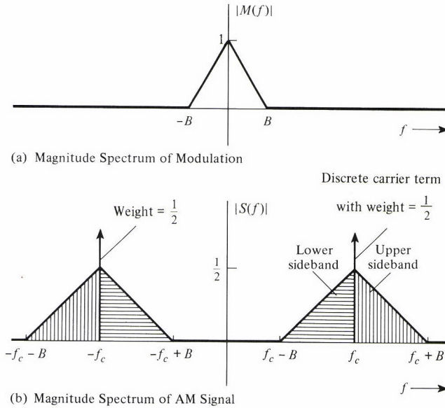
FIGURE 4-4 Spectrum of an AM signal.
