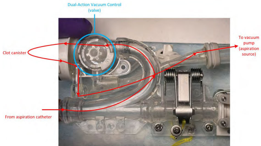
(Annotated image of Symphony housing (internal).)
