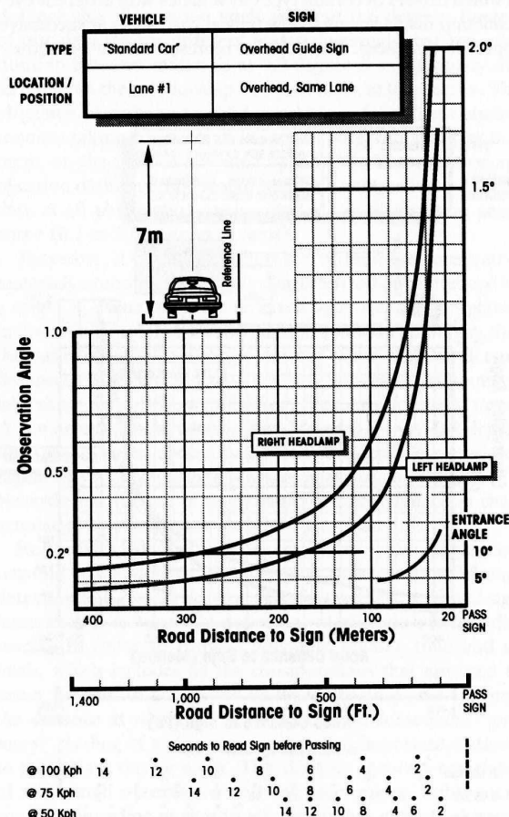
FIGURE 4 Observation angle versus road distance for overhead guide signs. Entrance angle shown where 5 degrees or more (to lower right vertical scale).
