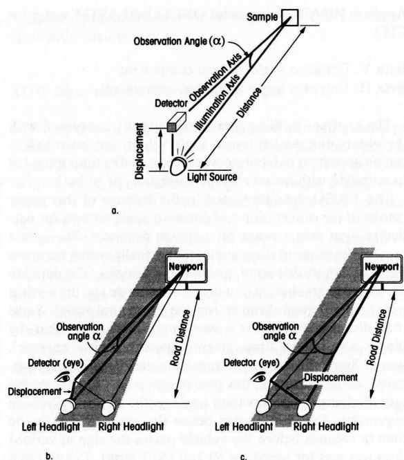
FIGURE 1 Observation angle: (a) laboratory test setup per specifications; (b) road to left headlamp; (c) road to right headlamp.
