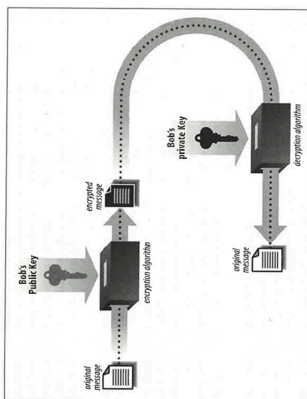
Figure 1-2. Public key cryptography
