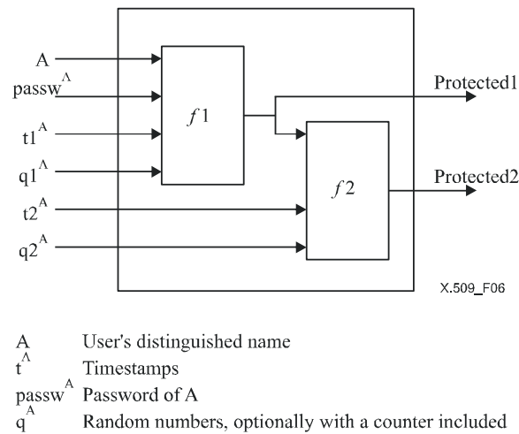
Figure 6 – Protected simple authentication
