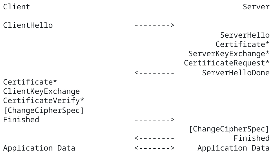
Figure 1. Message flow for a full handshake
