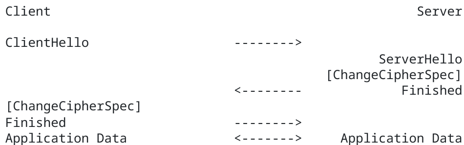
Figure 2. Message flow for an abbreviated handshake
