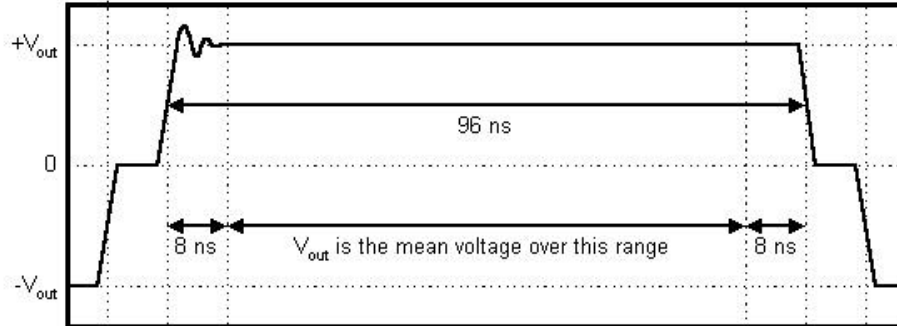
Figure 25.1.1-1: Differential output voltage reference waveform
