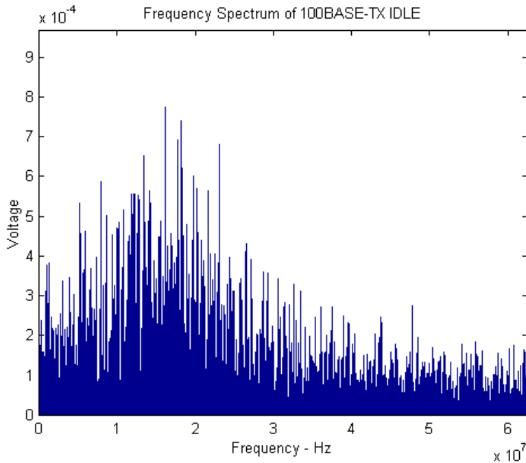
Figure 25.E-1 – Frequency Spectrum of 100Base-Tx IDLE
