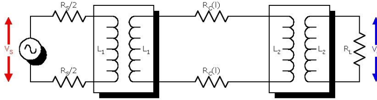
Figure 25.C-2: Baseline wander circuit model
