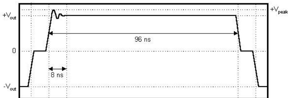
Figure 25.1.5-1: Waveform overshoot reference waveform
