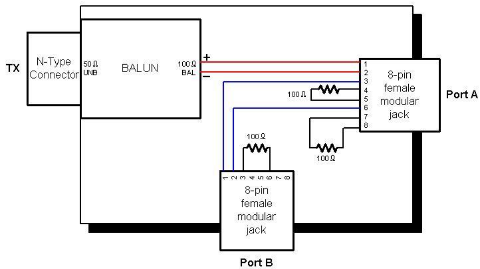
Figure 25.A-8: Test jig #2
