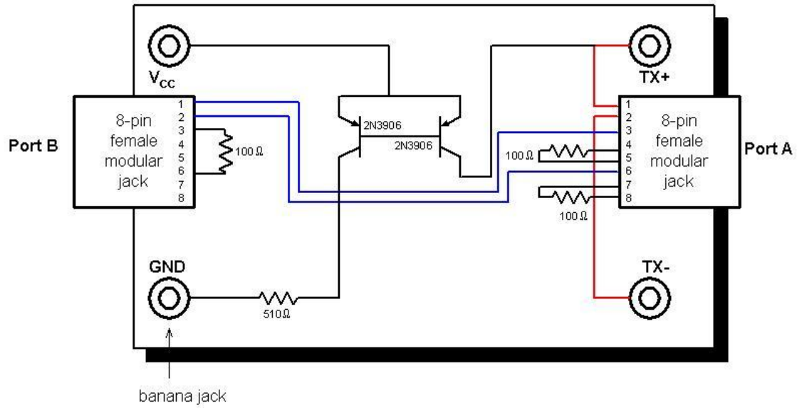
Figure 25.A-9: Test jig #3
