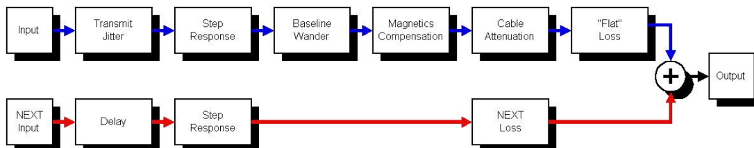
25.C-1: Link model block diagram
