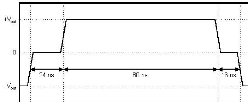
Figure 25.1.2-1: Rise and fall time reference waveform.
