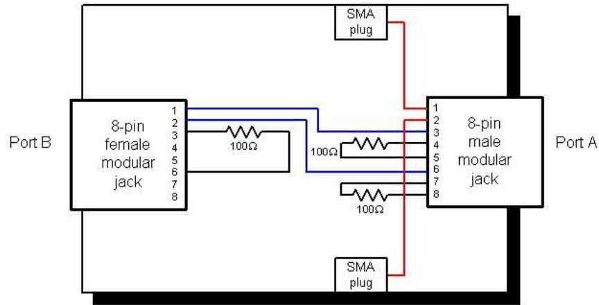
Figure 25.A-7: Test jig #1
