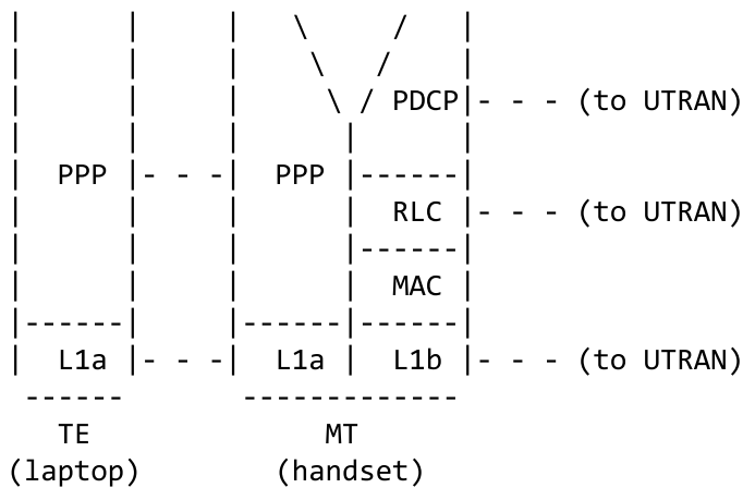
Figure 3: Laptop Attached to 3GPP Handset
