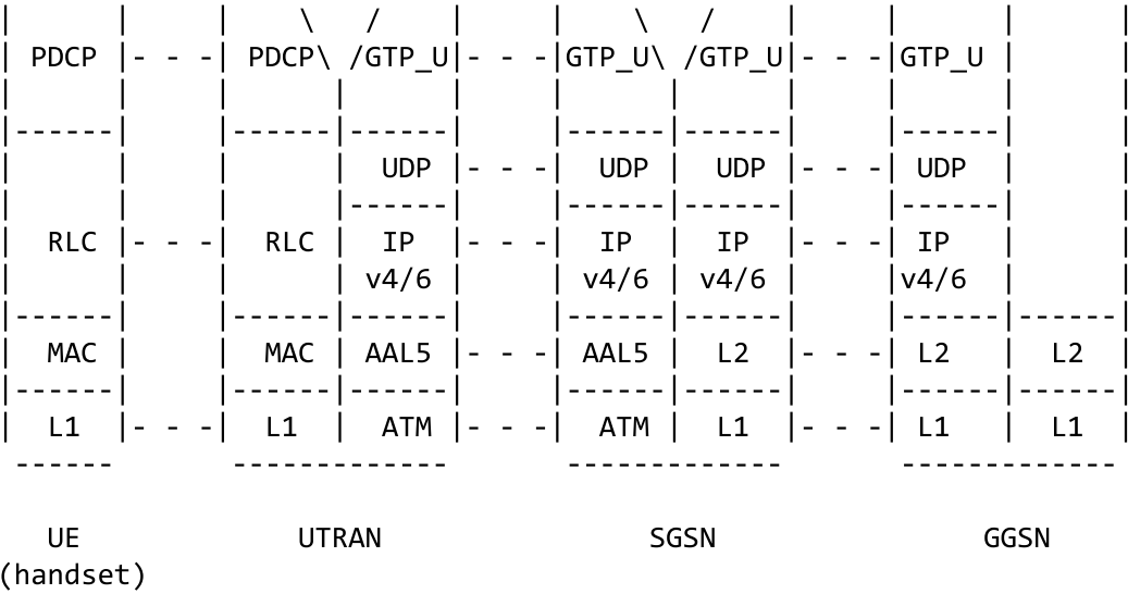
Figure 2: GPRS Protocol Stacks
