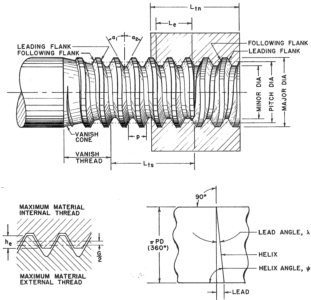
FIGURE 1.2. General screw thread symbols (see table 1.4).
