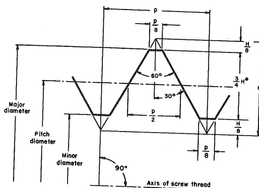
FIGURE 2.2. Basic unified thread form; ISO basic profile and American (U.S.) symmetrical thread form.
