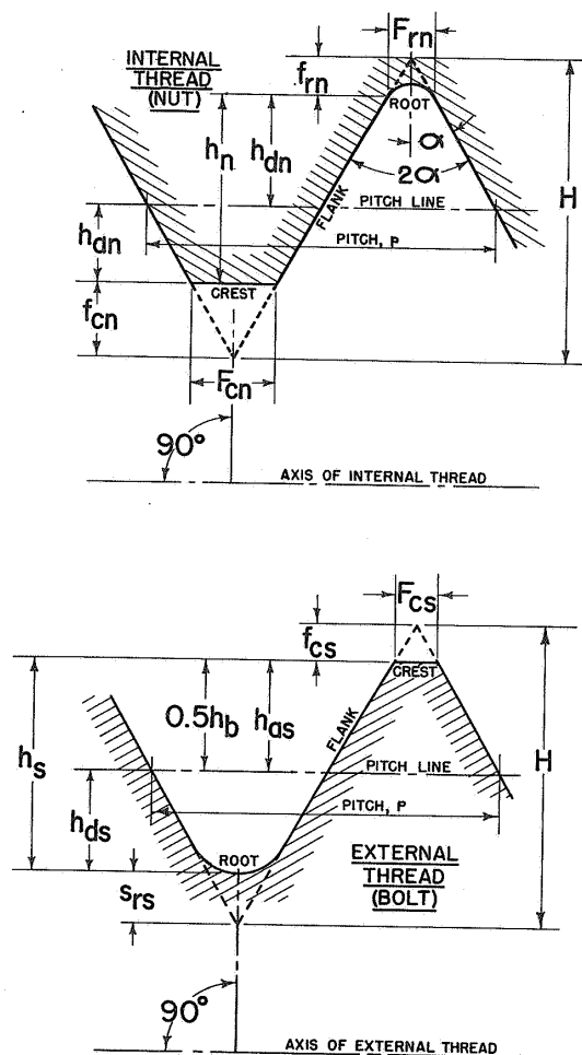
FIGURE 2.4. Symbols for thread data in table 2.1.
