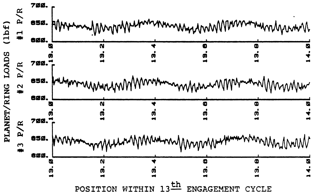
Figure 34 - Planet Loading at Pseudo-Static Conditions
