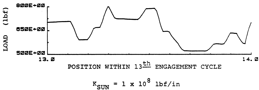
Figure 31 - Effect of Sun Support Stiffness on Planet Load
