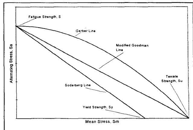
Figure 7 - Goodman Diagram
