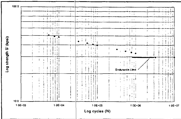
FIGURE 5. SN Diagram
