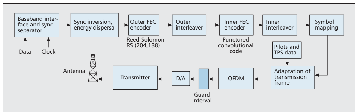
Figure 16. The DVB-T system [34].
