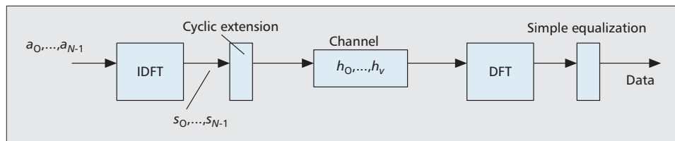
Figure 6. OFDM system.
