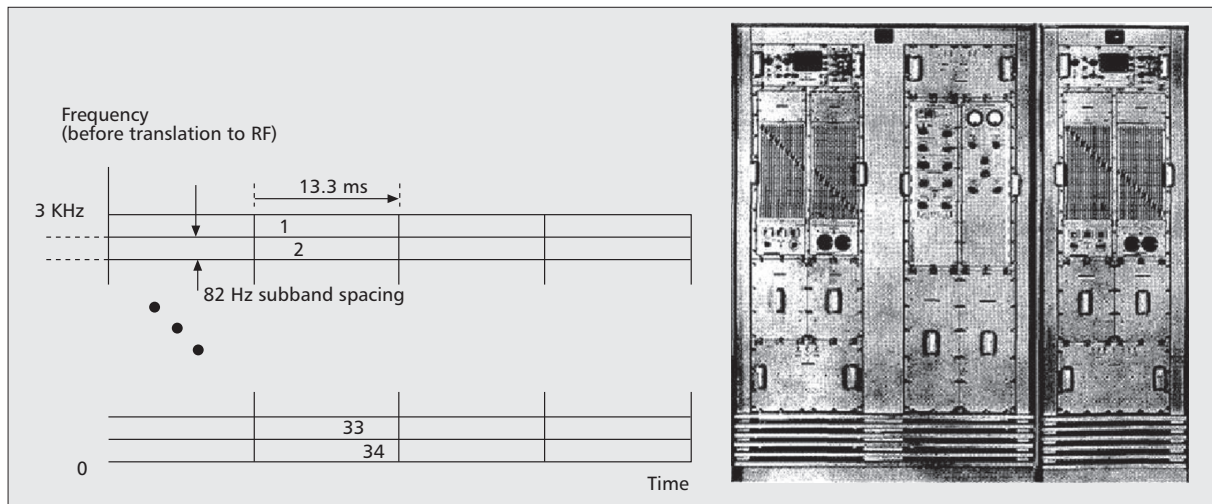
Figure 10. The 1967 KATHRYN high-frequency radio OFDM system [13].
