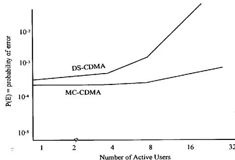
Figure 6. Representation of P(E) of DS-CDMA and MC-CDMA. Results are representative of those in [19].
