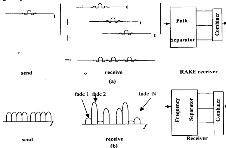
Figure 5. Multipath effects and receivers when processed in (a) time and (b) frequency
