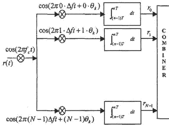
(b) receiver for user k
