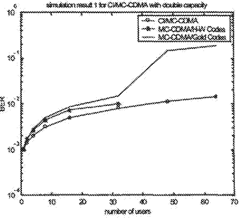
Figure 4: Simulation result 1, HT channel, SNR=10dB
