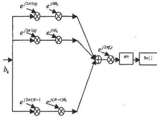
(a) transmitter for user k
