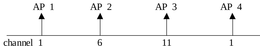
Figure 4: Initial channel autoselection, for a band of 14 channels
