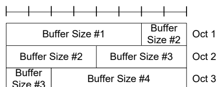
Figure 6.1.3.1-2: Long BSR MAC control element
