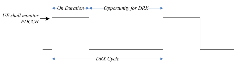
Figure 3.1-1: DRX Cycle
