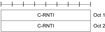
Figure 6.1.3.2-1: C-RNTI MAC control element
