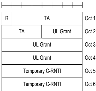
Figure 6.1.5-3: MAC RAR
