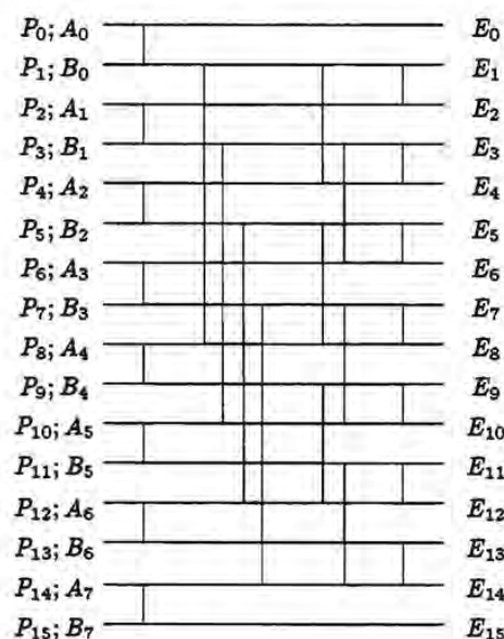
Figure 1. Odd-even merge with 16 processors.
