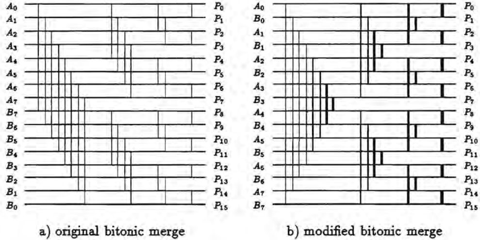
Figure 4. Bitonic merge with 16 processors.
