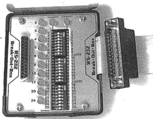
Breakout box.
