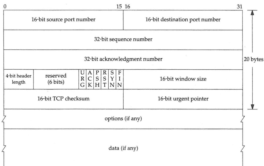
Figure 17.2 TCP header.
