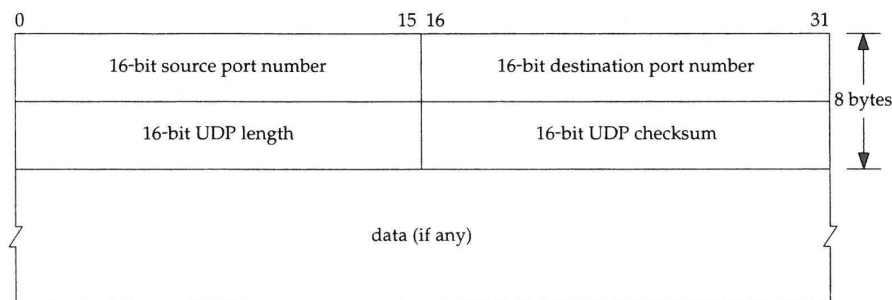
Figure 11.2 UDP header.
