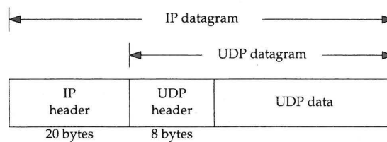
Figure 11.1 UDP encapsulation.
