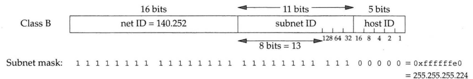
Figure 3.11 Using variable-length subnets.
