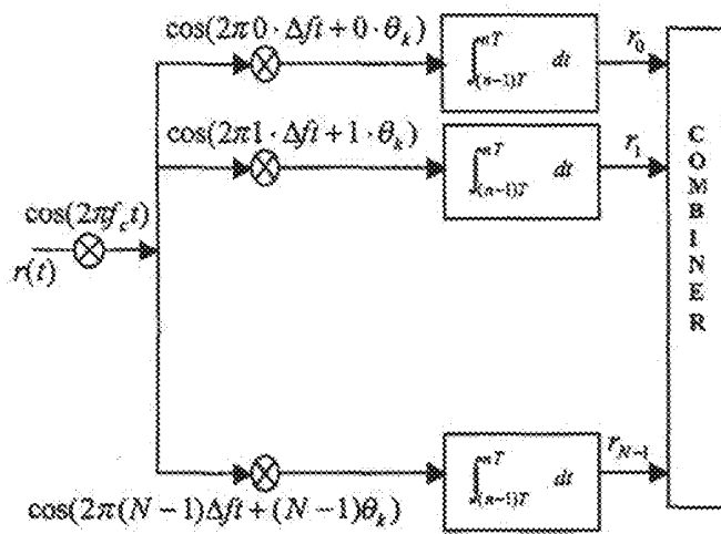
(b) receiver for user k
