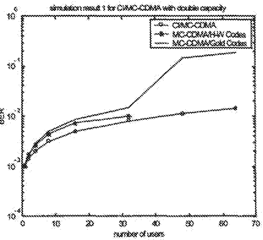
Figure 4: Simulation result 1, HT channel, SNR=10dB
