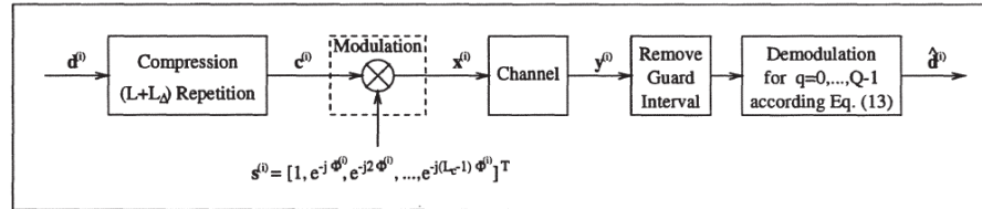
Figure 1: Block diagram of the proposed IFDMA system
