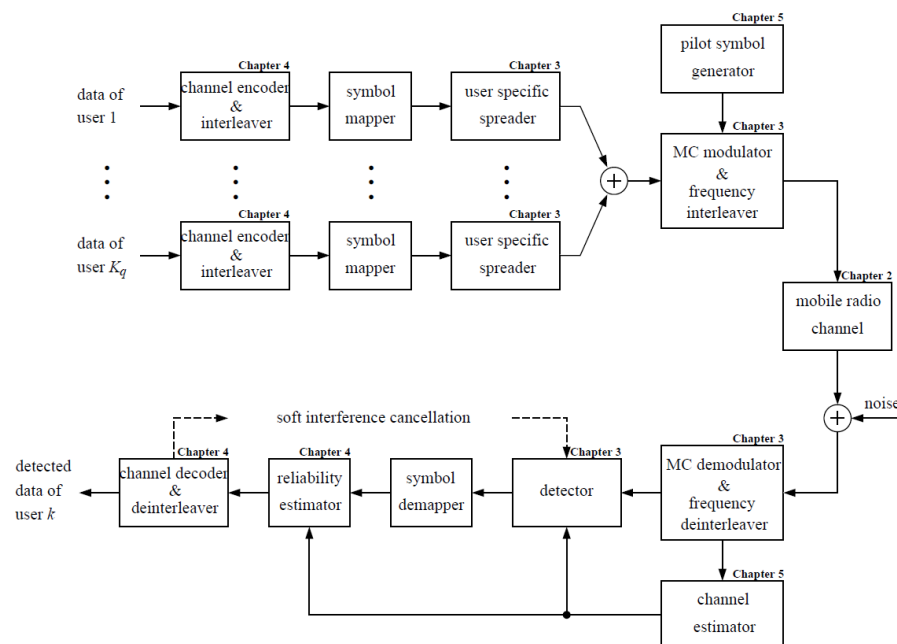
Figure 6.1: MC-CDMA mobile radio system in the downlink
