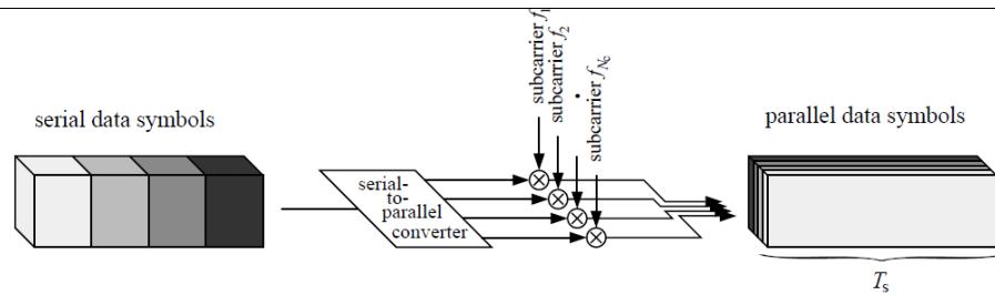
Figure 1.3: Principle of multi-carrier modulation; T_s = T_d N_c
