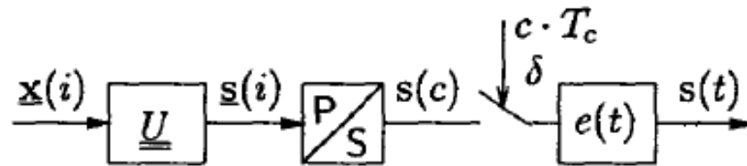
Fig. 2. Equivalent transmitter model.
