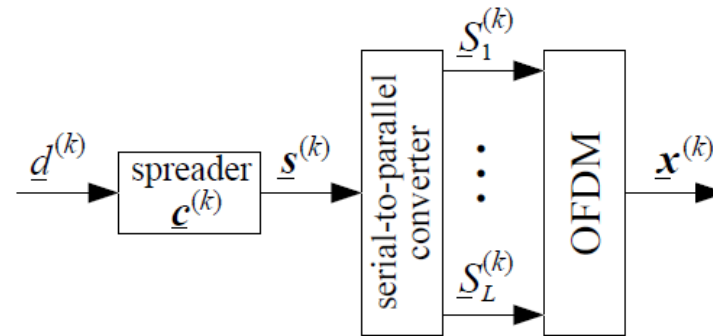
Figure 3.6: MC spread spectrum signal generation
