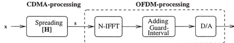
Figure 1: Block diagram of a MC-CDMA transmitter (downlink)
