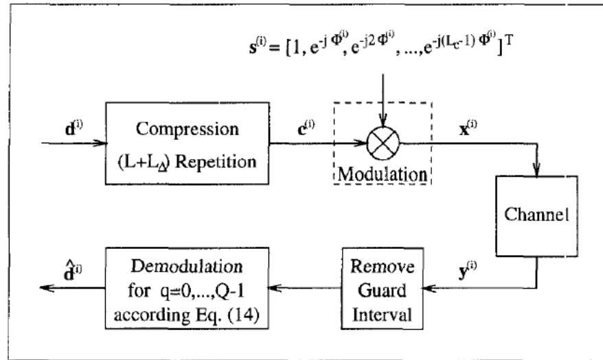
Figure 2: Block diagram of the proposed IFDMA system for a single user i
