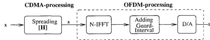
Fig. 1. Block diagram of a multi-carrier CDM transmitter
