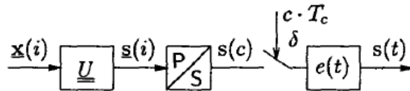
Fig. 2. Equivalent transmitter model.
