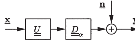
Figure 4 Transmission over non-interfering channels with orthogonal spreading
