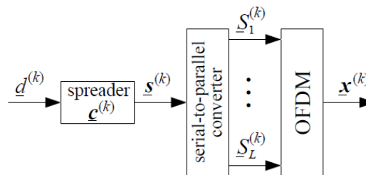
Figure 3.6: MC spread spectrum signal generation
