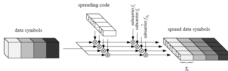
Figure 1.4: Principle of spreading of the data of a single user by MC-CDMA for the case N_c = L , i.e., T_s = T_d and T'_c = T_d
