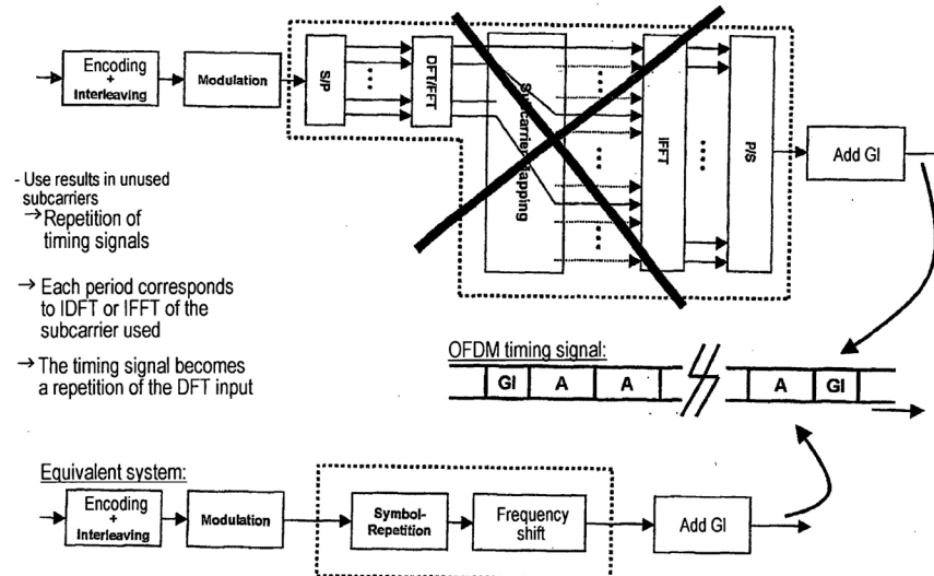
FIG 4: OFDM-FDMA Uplink (only one user sending)
