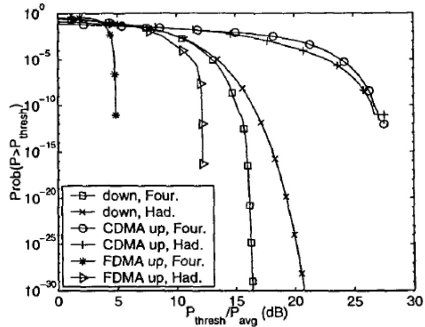
Fig. 4. Example for amplitude distribution.
