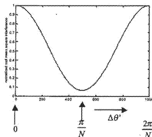
Figure 2: Root Mean Square Cross Correlation versus \Delta\theta'
