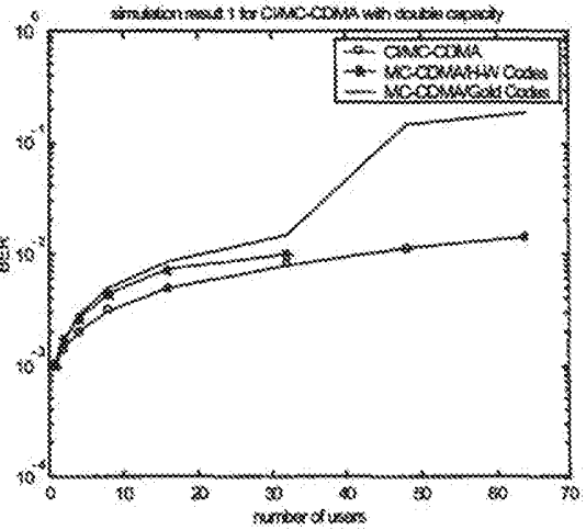
Figure 4: Simulation result 1, HT channel, SNR=10dB
