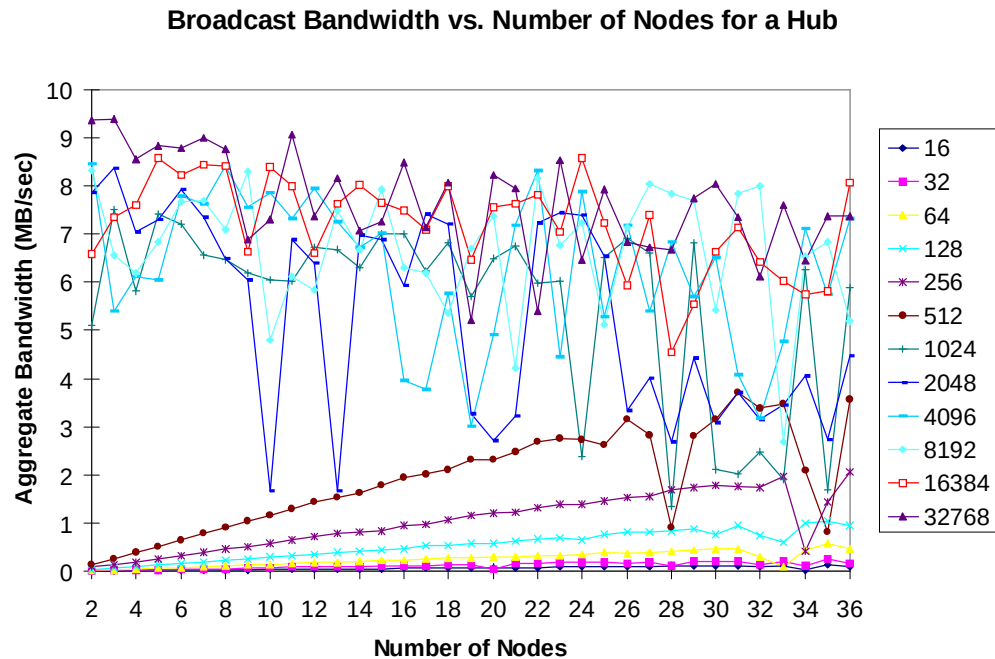
FIGURE 10. Collective communication performance on a hub
