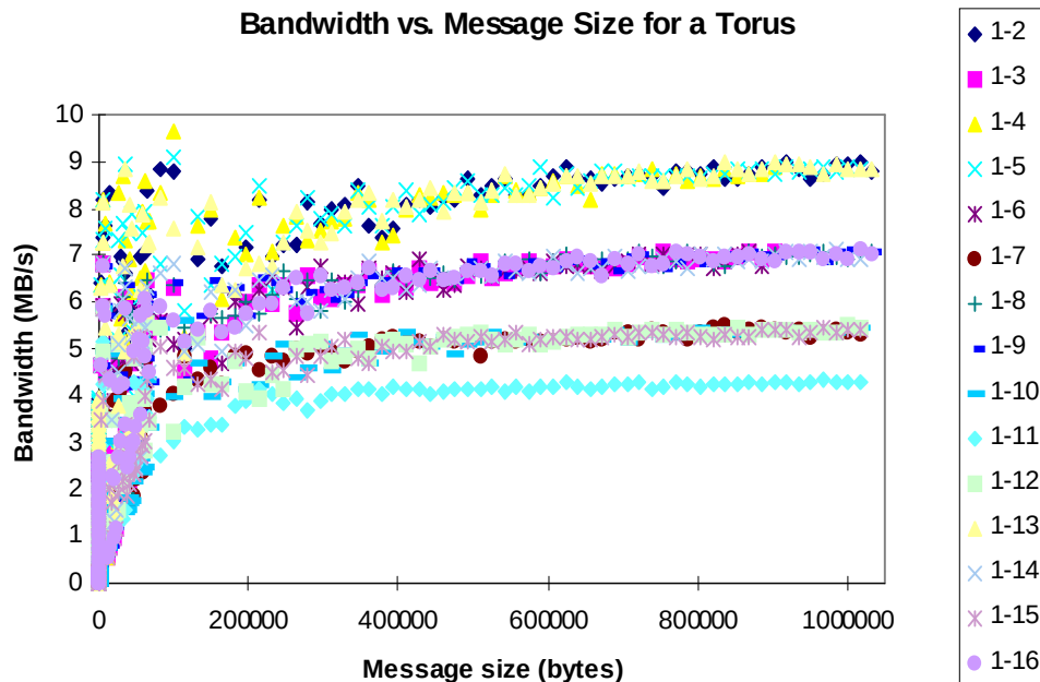
FIGURE 7. Bandwidth performance of the torus topology
