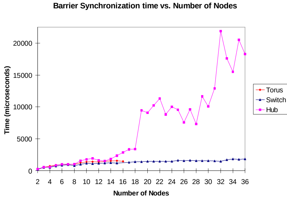
FIGURE 12. Comparison of barrier synchronization time for the hub, switch, and torus
