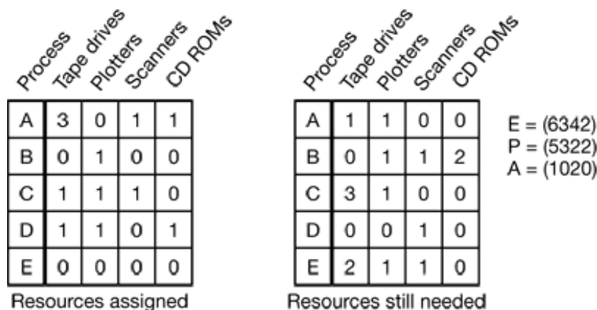
Figure 3-12. The banker's algorithm with multiple resources.
