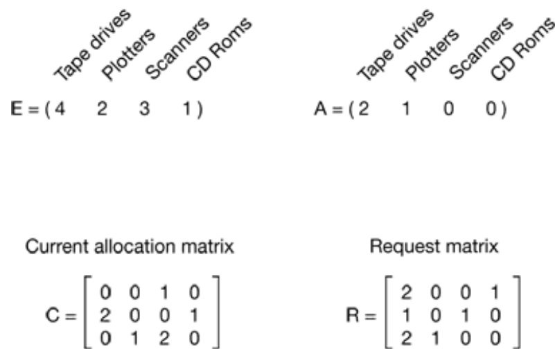
Figure 3-7. An example for the deadlock detection algorithm.
