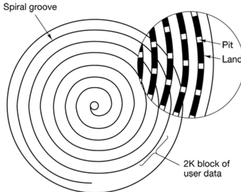
Figure 5-20. Recording structure of a compact disc or CD-ROM.
