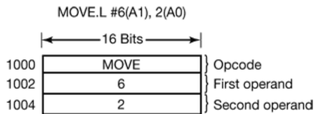
Figure 4-32. An instruction causing a page fault.
