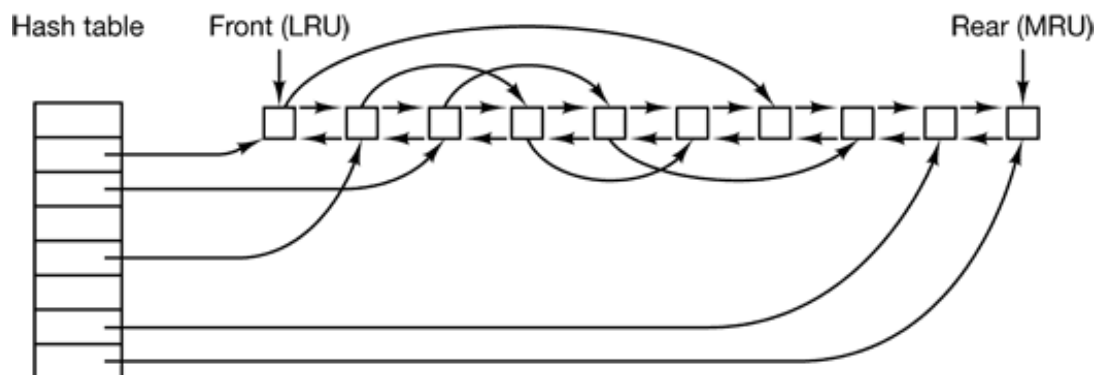
Figure 6-27. The buffer cache data structures.
