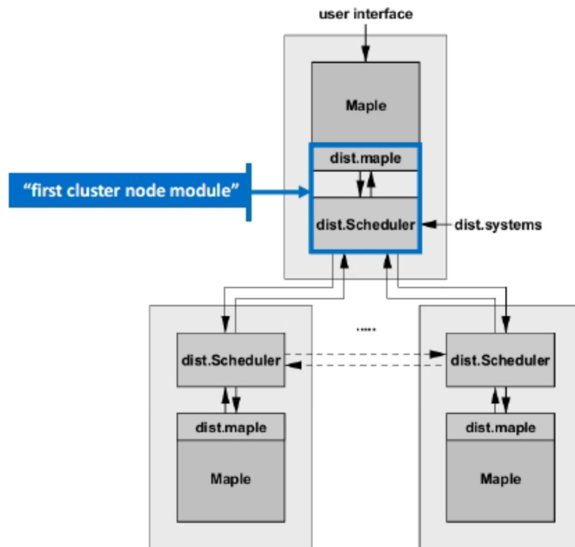
Fig. 1. Software architecture.
