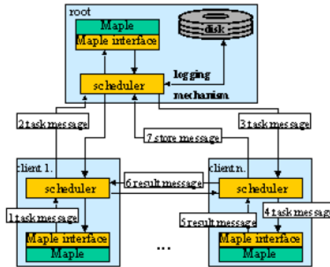
Figure 1: Execution Model
