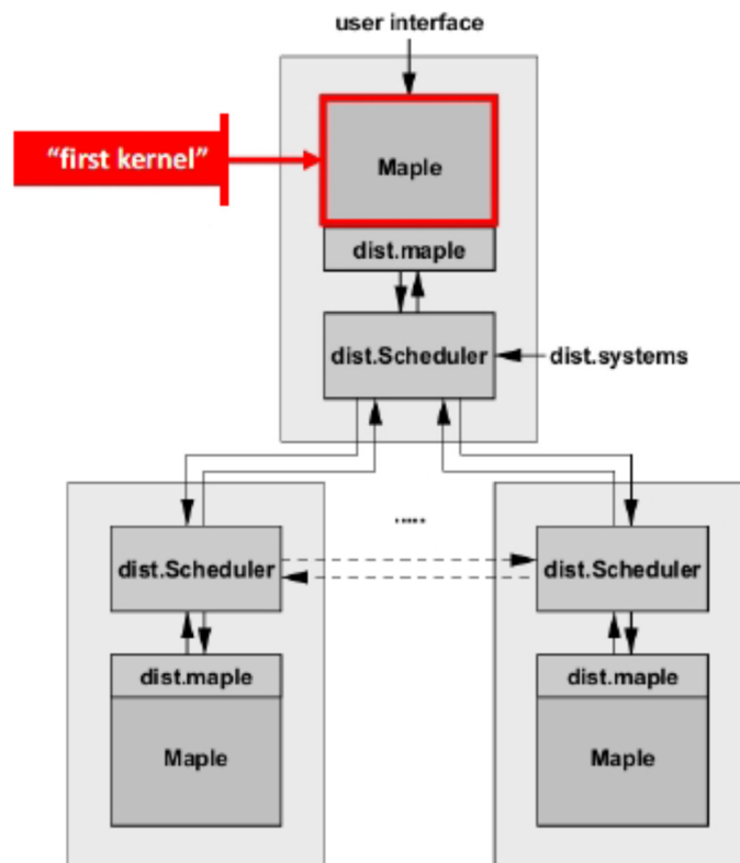
Fig. 1. Software architecture.
