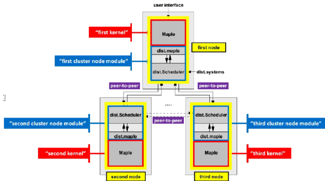
Fig. 1. Software architecture.
