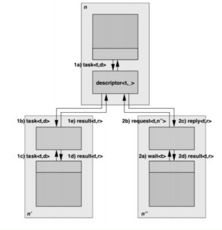
Figure 5 of Schreiner1 is an “execution model” of Distributed Maple. Ex. 1108, 320.
