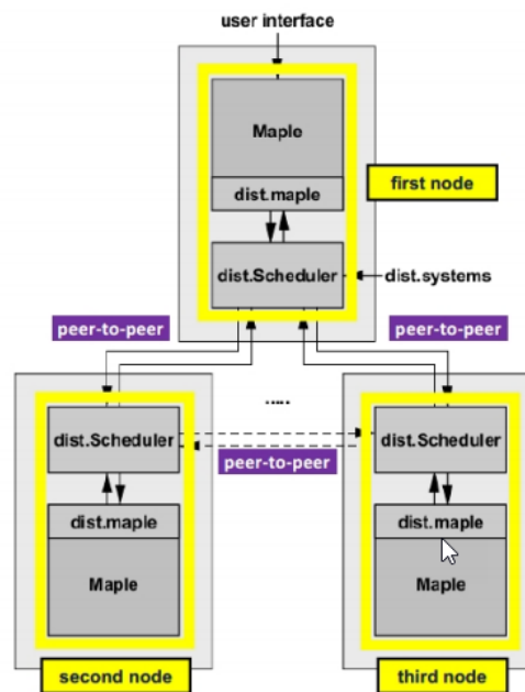
Fig. 1. Software architecture.
