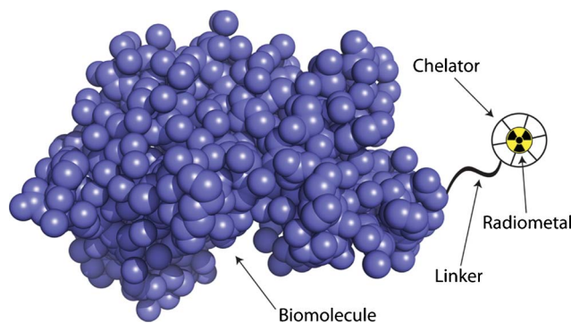
Fig. 1 The anatomy of a PET bioconjugate.
