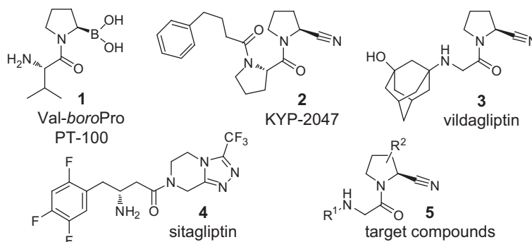
Figure 1. Reference compounds used in this study (1–4) and generic structure of products reported in this publication (5).
