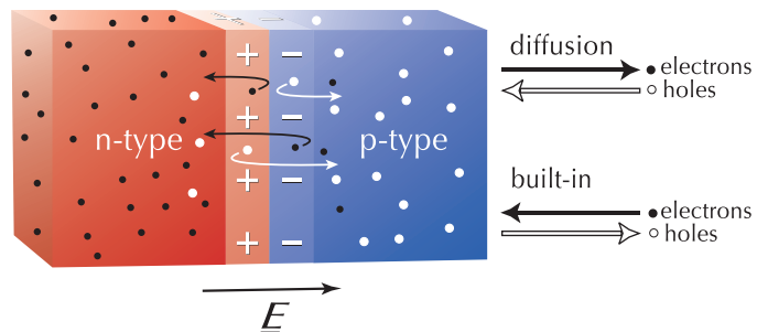
Figure 4 Motion of mobile electrons and holes due to diffusion and the "built-in" electric field.
