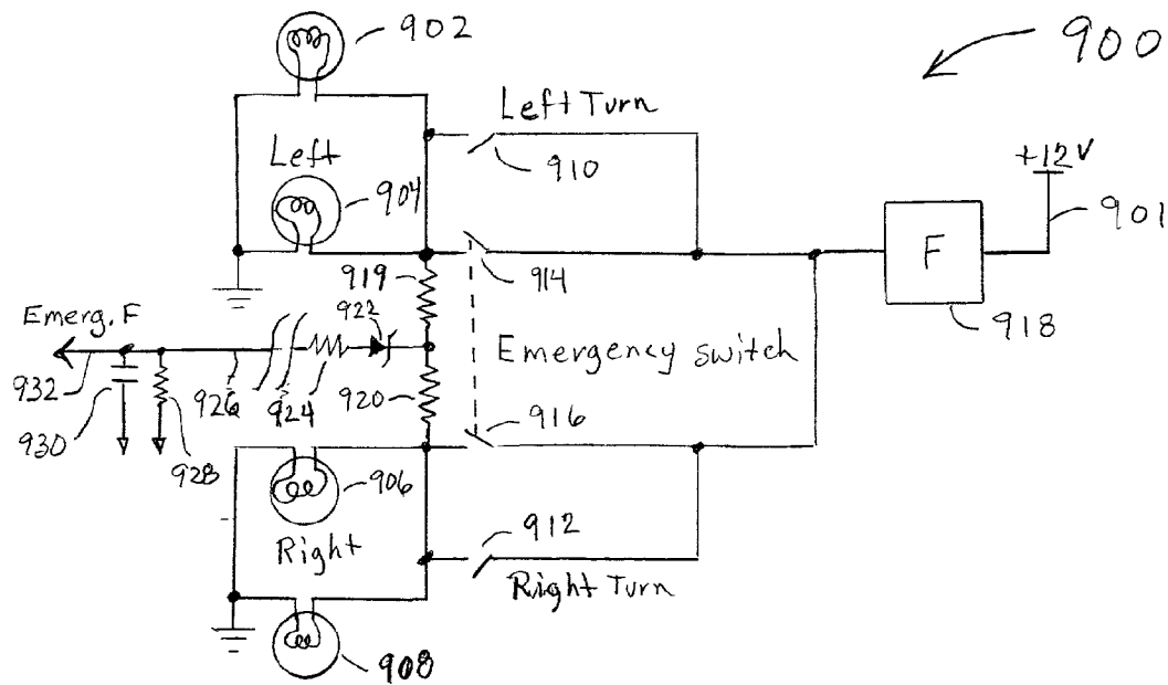
FIG. 18 Emergency Flasher Sense
