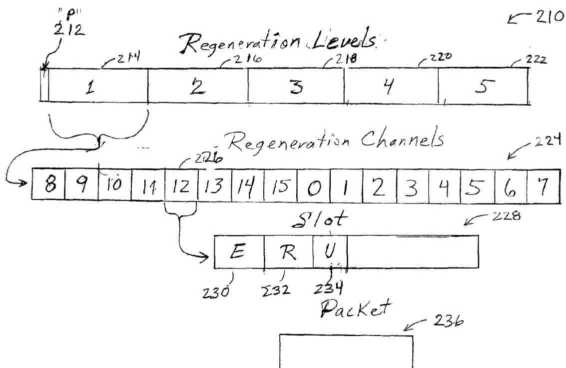
FIG. 6 Regeneration Scheme Division
