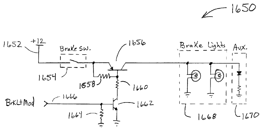
FIG. 35 Brake Light Modulation Circuit
