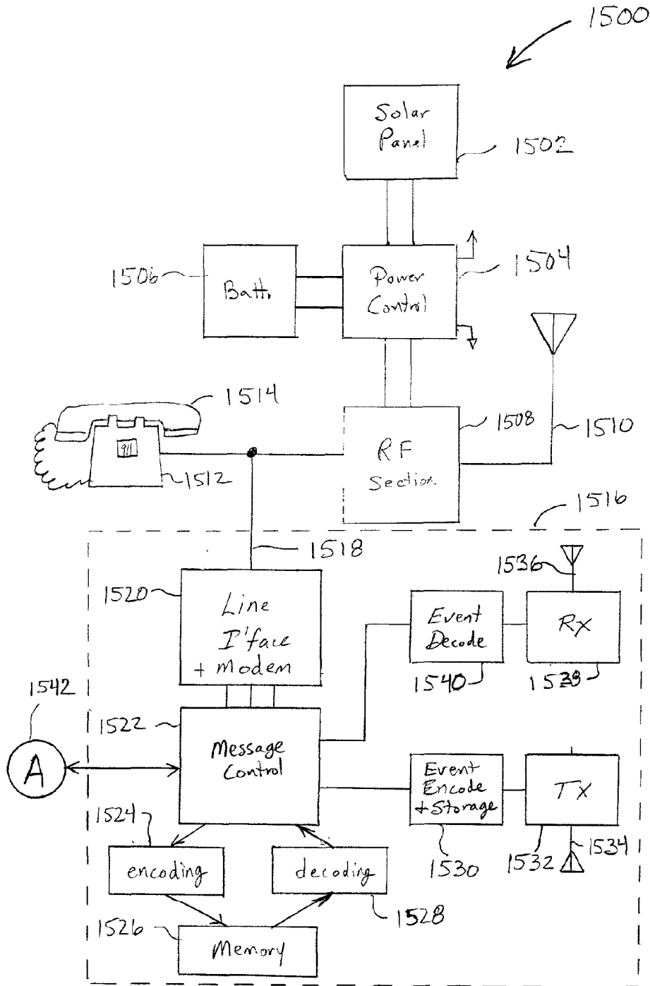
FIG. 30 HBC Call Box Interface
