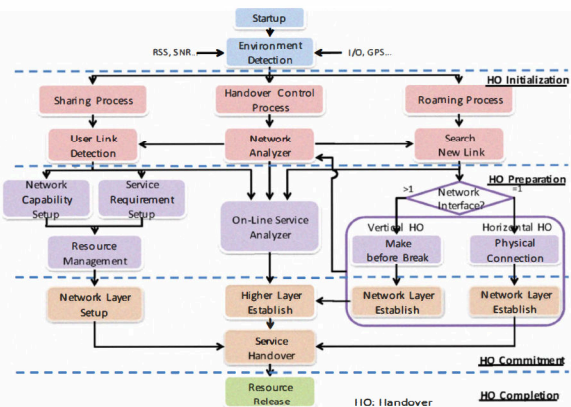
Figure 2. The flowchart of heterogeneous network management
