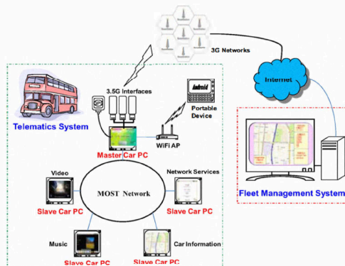
Figure 6. Android system integrated with MOST networks
