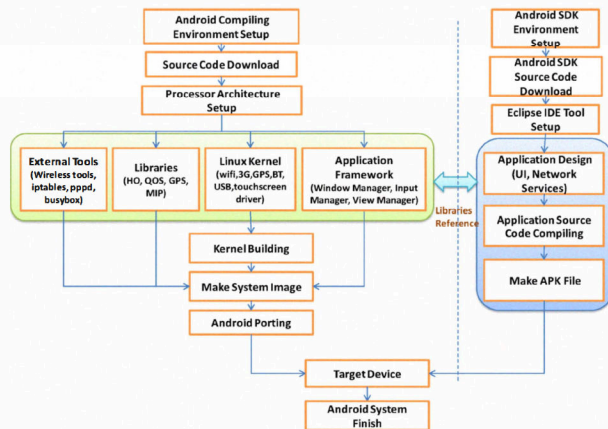
Figure 3. Android system implementation flowchart
