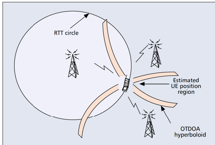
■ Figure 3. OTDOA positioning method.
