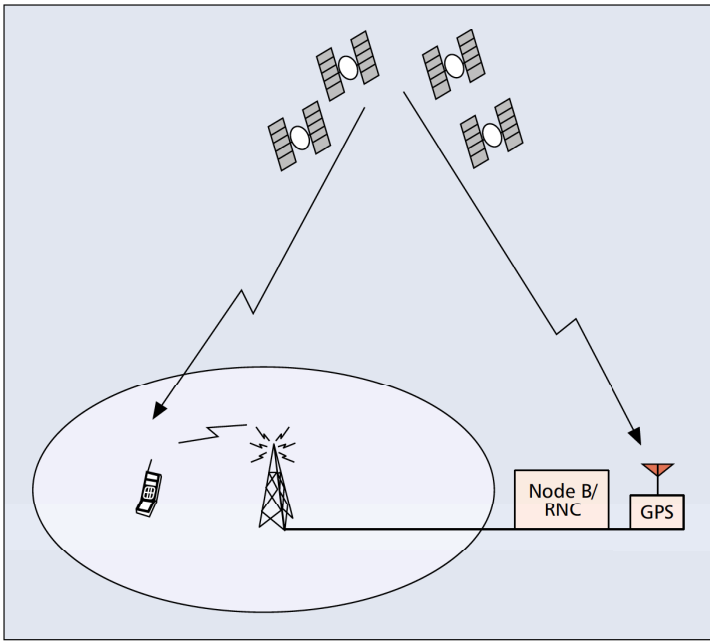
■ Figure 4. Assisted GPS positioning method.
