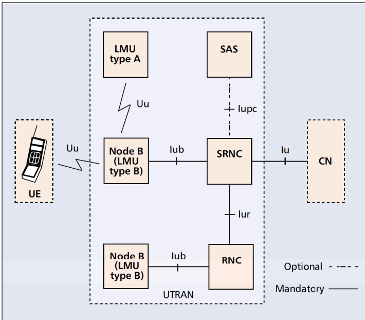
■ Figure 2. System architecture of UE positioning.
