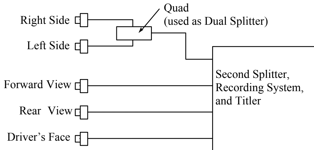
Figure 2.8. Video Diagram Showing Use of Quad Splitters.
