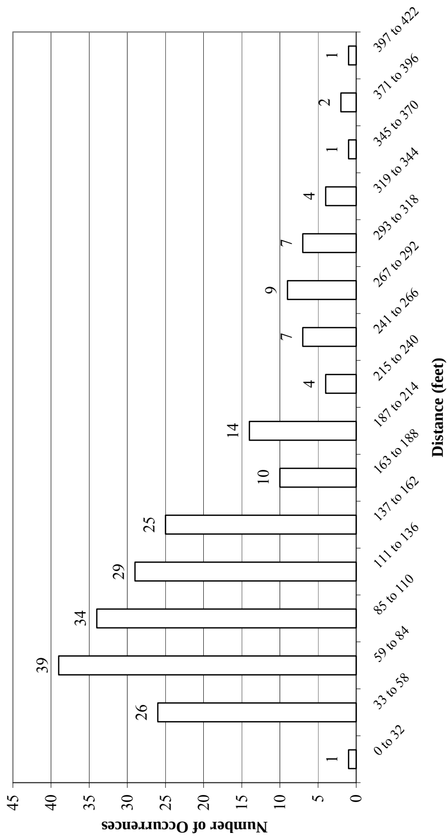
Figure 4.33. Frequency Distribution of Distance to Closest Rearward Vehicle at t_0 ( N = 213 ).
