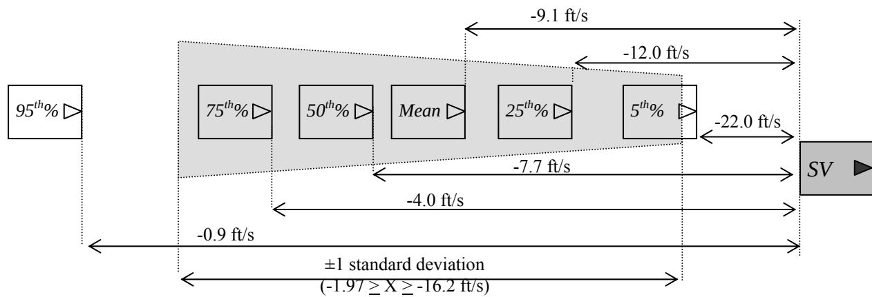
Figure 4.46. Percentile Relative Velocity to Closest Rearward Vehicle Relative to SV at t_0 . (This diagram is a depiction of data and is not geometrically accurate.)
