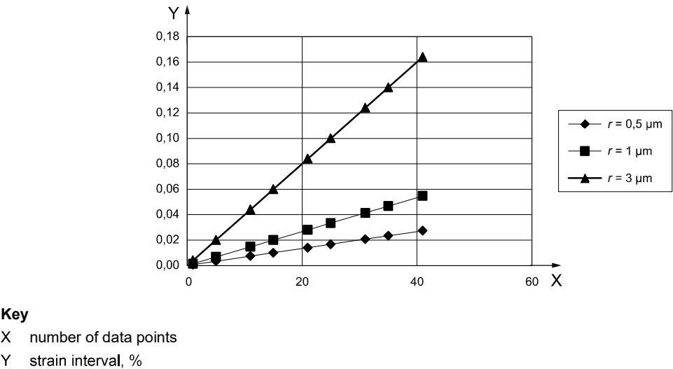
Figure A.1 — Strain interval according to Equation (A.2)
