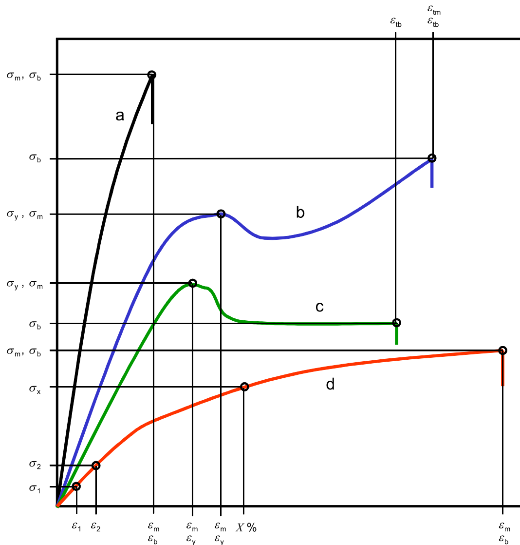
Figure 1 — Typical stress/strain curves
