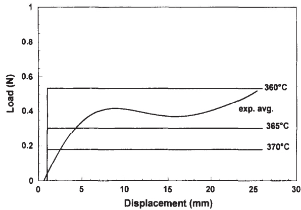
Figure 9 Experimental and predicted load histories for tests conducted at 2.12 mm/s on [0/90/\pm 45]_{2s} specimens
