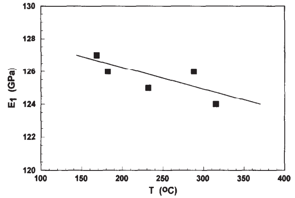
Figure 2 Temperature dependence of E_1 above the glass transition temperature for AS4/PEEK
