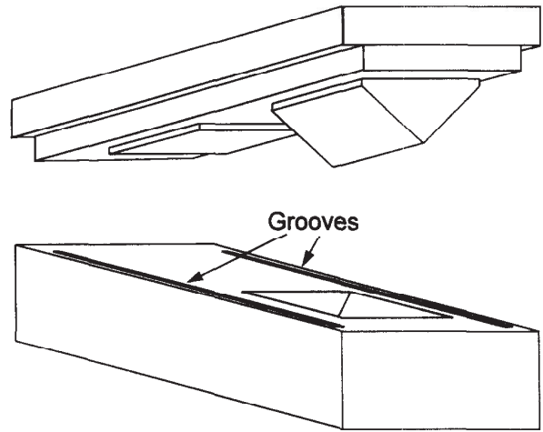
Figure 11 Two-stage matched die mold with right angle forming cavity
