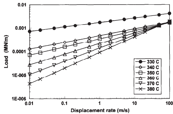
Figure 5 Variation of the load required to maintain a given displacement rate with temperature for the concentrated load forming example
