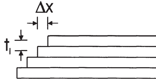
Figure 1 One-dimensional ply slip relationship
