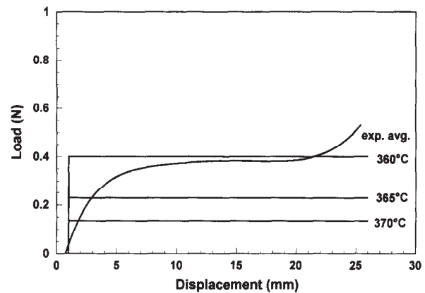
Figure 7 Experimental and model load histories for tests conducted at 2.12 mm/s on [0/90]_{3s} specimens
