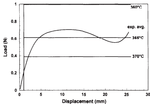
Figure 10 Experimental and predicted load histories for tests conducted at 8.47 mm/s on [0/90/\pm 45]_{2s} specimens
