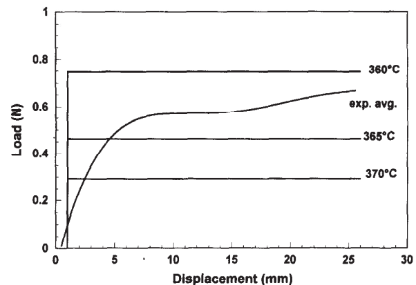
Figure 8 Experimental and predicted load histories for tests conducted at 8.47 mm/s on [0/90]_{3s} specimens
