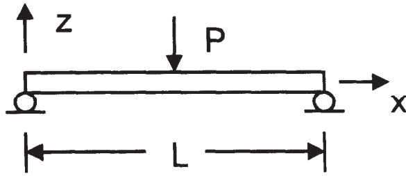
Figure 4 A simply supported, symmetric, cross-ply laminate subject to a concentrated load at mid-span
