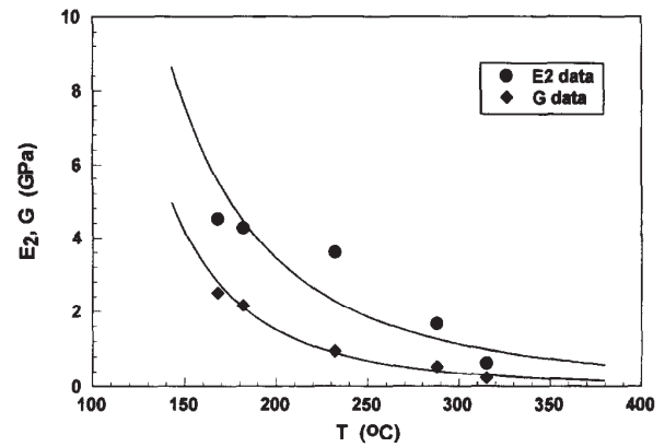
Figure 3 Temperature dependence of E_2 and G_{12} above the glass transition temperature for AS4/PEEK
