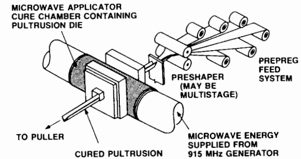
Figure 1-18 Pultrusion
