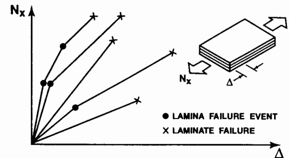
Figure 7-57 Effect of Changing Laminate Stacking Sequence
