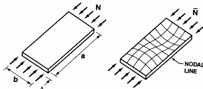
Figure 5-19 Typical Simply Supported Plate Buckling Mode
