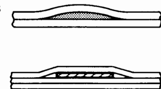
Figure 7-32 Padding Up
