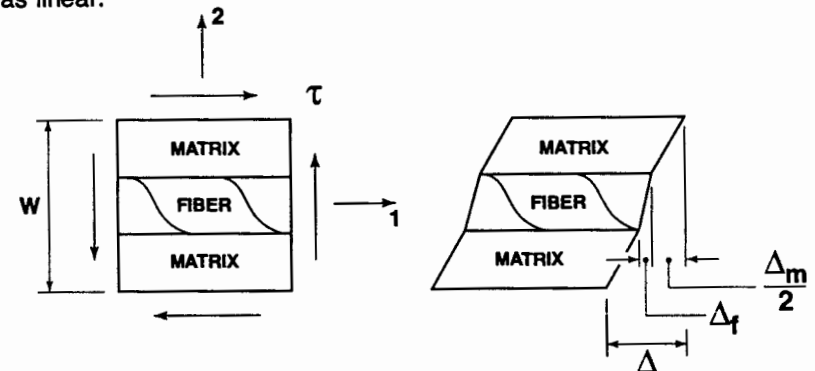
b Shear Deformation
