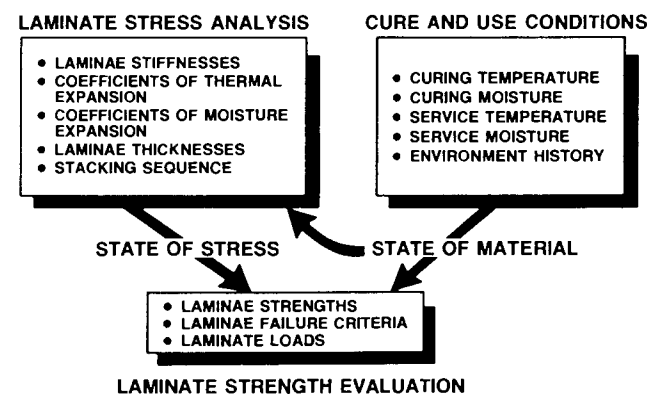
Figure 4-35 Laminate Strength-Analysis Elements
