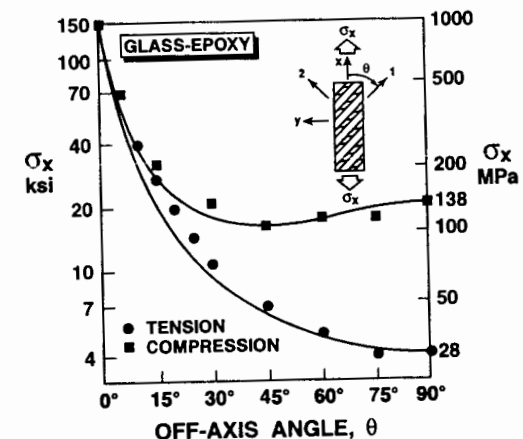
Figure 2-42 Hoffman Failure Criterion for Glass-Epoxy (Data from Tsai [2-21])
