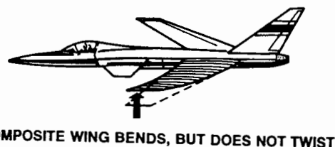
Figure 4-17 Response of Forward-Swept Wings
