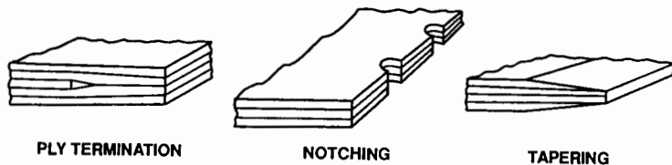
Figure 4-61 Free-Edge Delamination-Suppression Concepts
