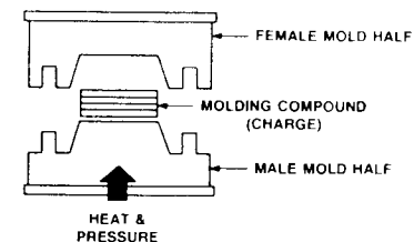
Figure 1-13 Compression Molding
