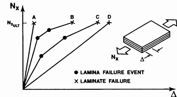
Figure 7-56 Possible Laminate Behaviors
