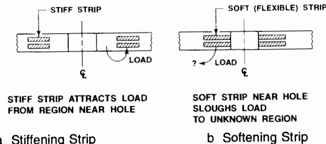
Figure 6-9 Concepts for Stress Concentration Reduction around Holes
