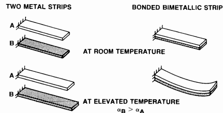
Figure 1-3 Cantilevered Bimetallic Strip (Thermostat)
