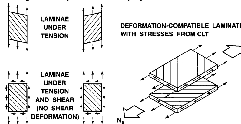
Figure 7-63 Laminate Free-Edge Stress State
