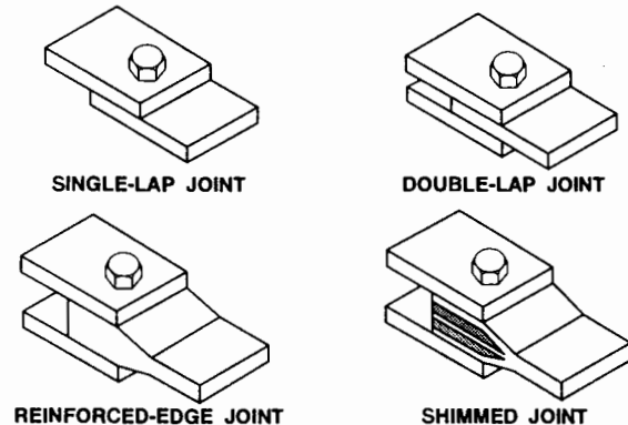
Figure 7-40 Bolted Joints
