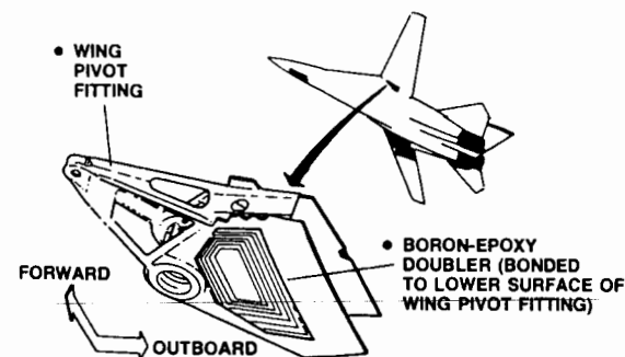
Figure 1-28 F-111 Wing-Pivot Fitting (Courtesy of Lockheed Martin)
