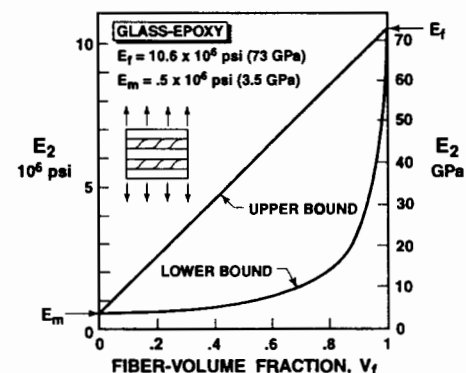
Figure 3-20 Bounds on E_2 for a Glass-Epoxy Composite Material
