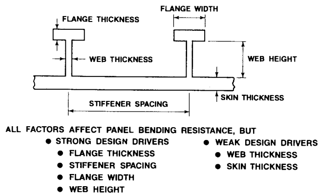
Figure 7-15 Anatomy of a Stiffened Panel
