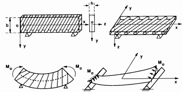
Figure 4-12 Effect of Bend-Twist Coupling on Plate Bending (After Ashton, Halpin, and Petit [4-3])
