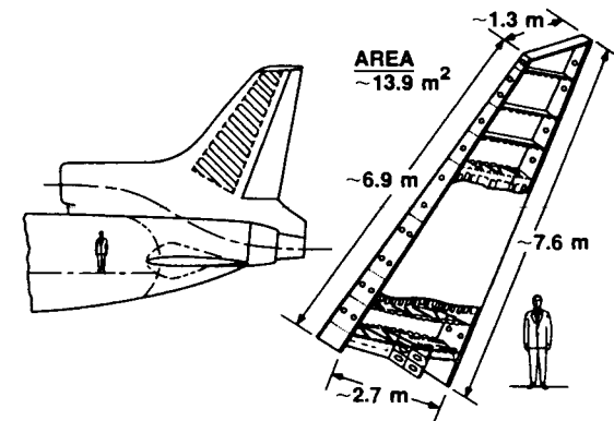
Figure 1-40 Lockheed L-1011 Vertical Fin (After Jackson, et al. [1-6])
