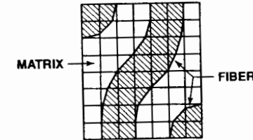
Figure 3-3 Finite Element Model of a Representative Volume Element for a Woven Lamina
