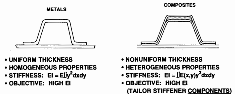
Figure 7-26 Metal Versus Composite Stiffener Characteristics
