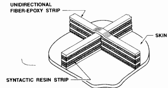
Figure 7-34 Orthogrid
