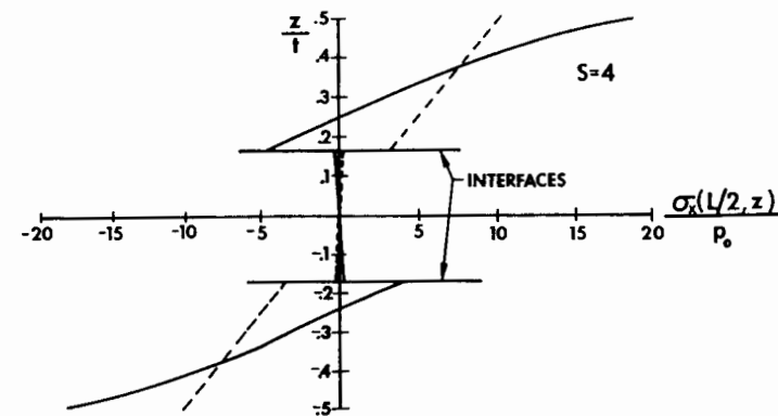
Figure 6-18a Variation of \sigma_x through the Thickness for S = 4 (After Pagano [6-21])
