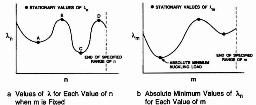
Figure 5-25 Determination of the Absolute Minimum Buckling Load
