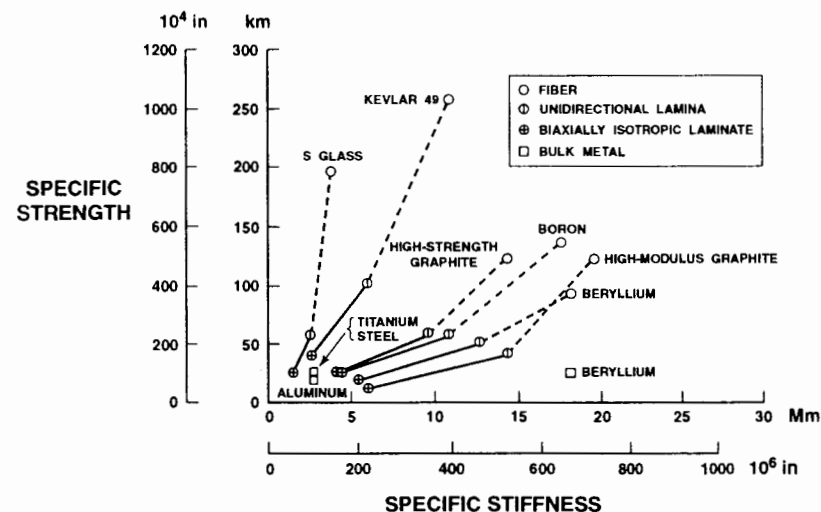
Figure 1-24 Strength and Stiffness of Composite Materials and Metals
