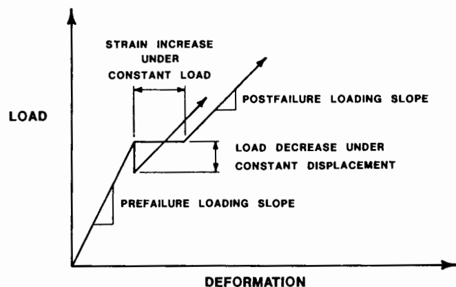
Figure 4-47 Behavior upon First-Layer Failure
