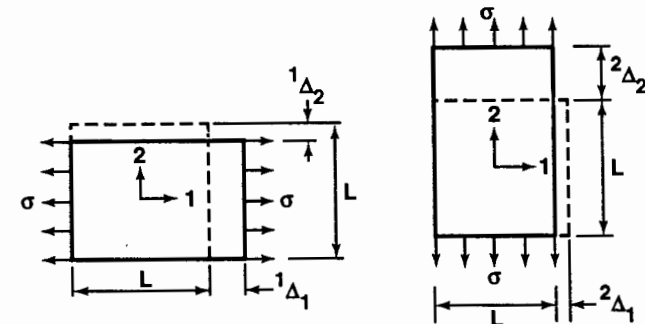
STRESS IN 1-DIRECTION
