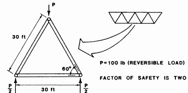
Figure 7-22 Space Truss Idealization
