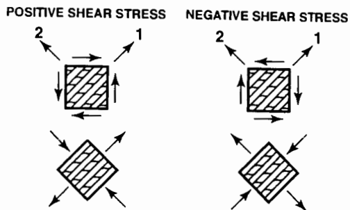
Figure 2-18 Shear Stress at 45^\circ to Principal Material Coordinates
