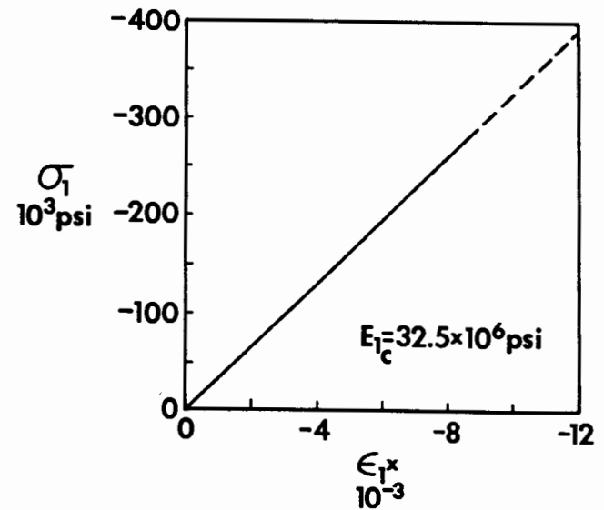
Figure C-7 Compressive \sigma_1 - \epsilon_1 Curve for Boron-Epoxy (Adapted from [C-2])
