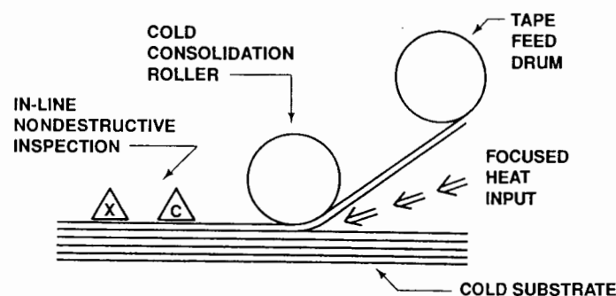
Figure 1-22 Thermoplastic-Matrix Layup and Curing Device
