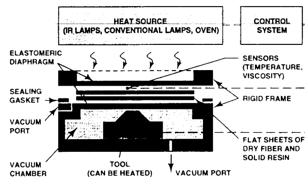
Figure 1-14 Resin-Transfer Molding
