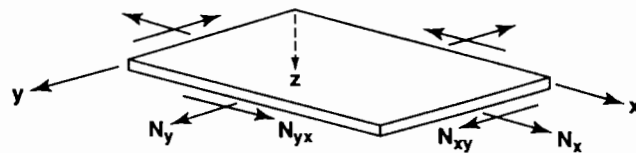
Figure 4-6 In-Plane Forces on a Flat Laminate
