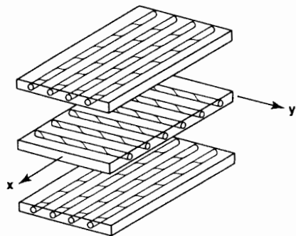
Figure 4-16 Unbonded View of a Three-Layered Regular Symmetric Cross-Ply Laminate
