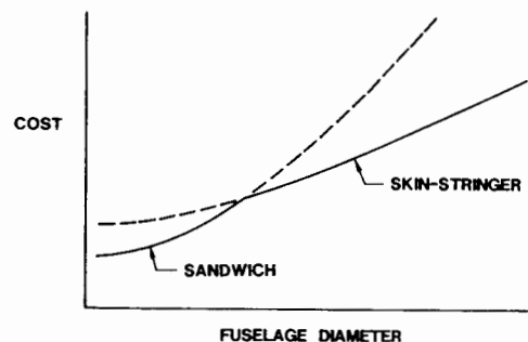
Figure 7-36 Configuration Trade-offs
