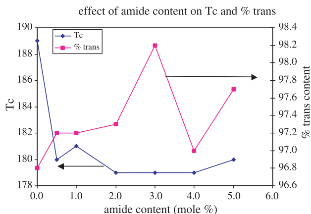
Fig. 12. The effect of amide content in PCCD copolymers on their glass transition temperatures, T_c and trans content of the diester in the polymer.
