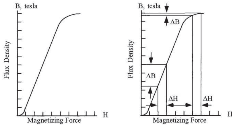
Figure 1-18. Magnetizing Curve.
