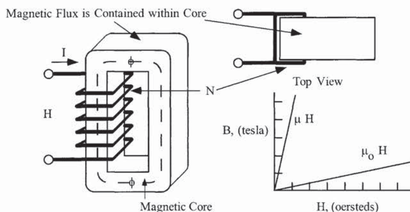
Figure 1-11. Introduction of a Magnetic Core.
