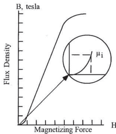
Figure 1-20. Initial Permeability.
